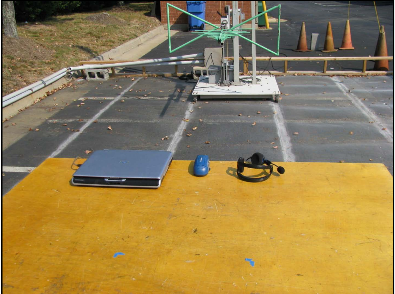
Photograph 1: Unintentional Radiated Emissions Testing – Front View
