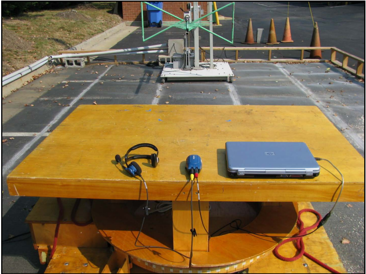
Photograph 2: Unintentional Radiated Emissions Testing – Back View
