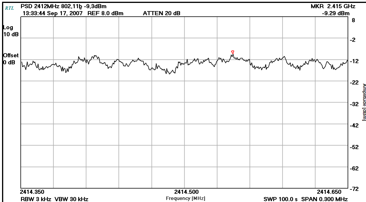
Plot 7-1: Power Spectral Density: Channel 1 (2412 MHz); 802.11b
