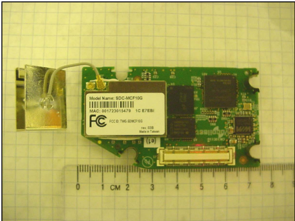
Photograph 8: Bottom of Top PCB Showing Radio with Shield and Antenna Connected
