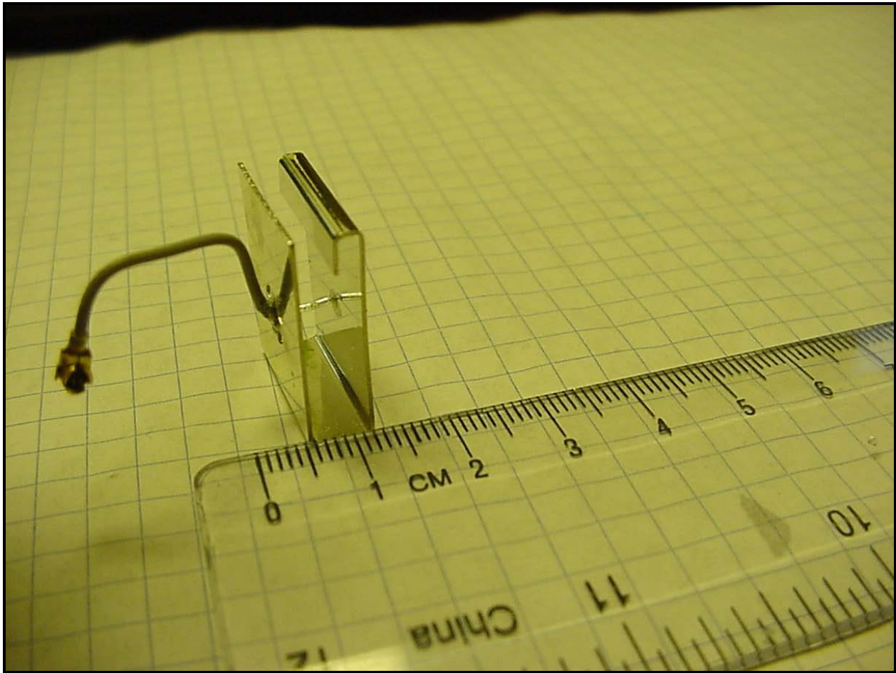
Photograph 11: Antenna
