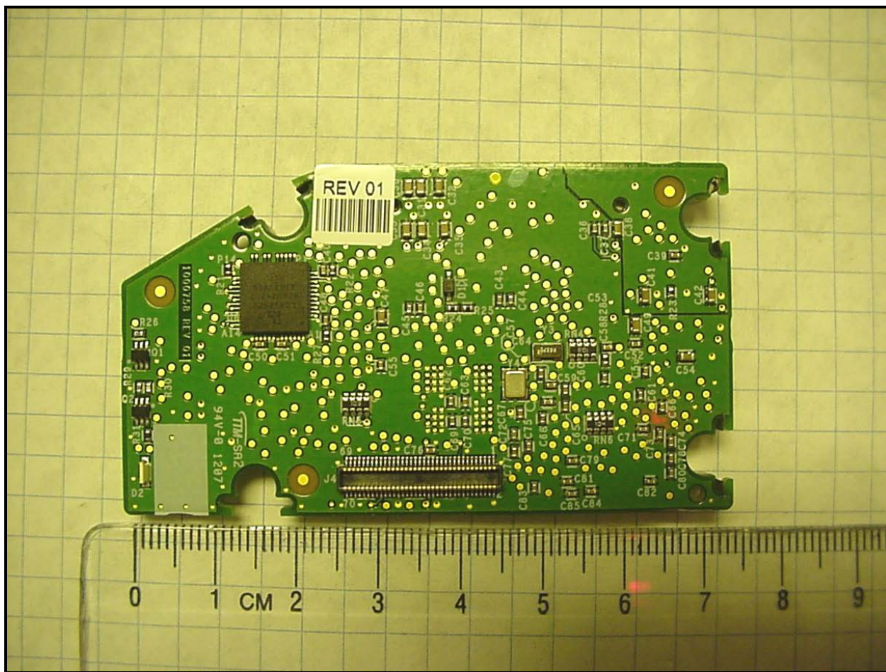
Photograph 10: Top of Front PCB
