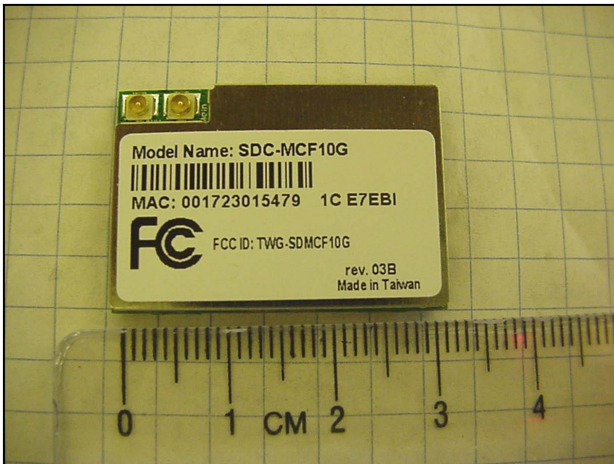
Photograph 13: Top of Radio Card with Shield
