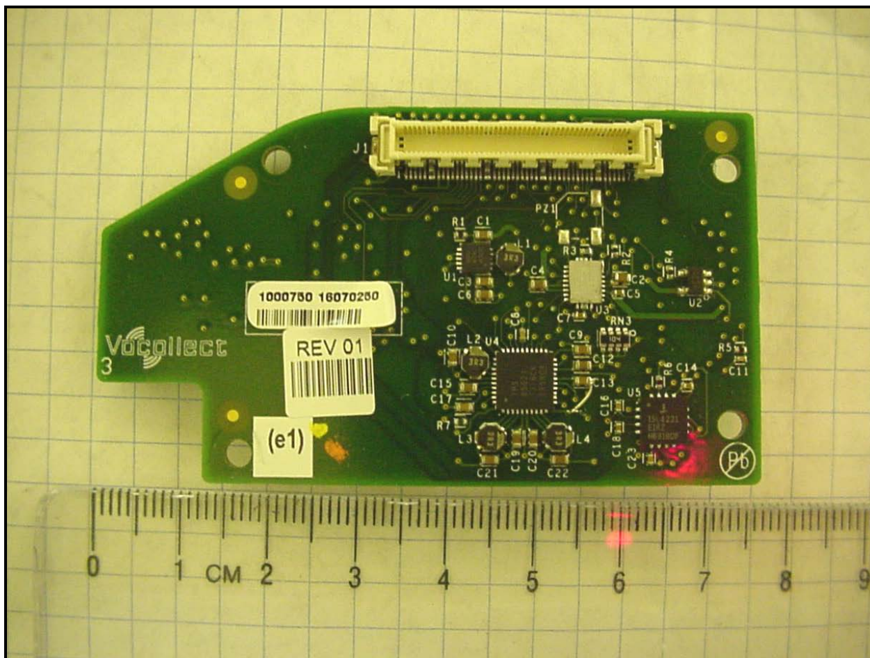
Photograph 7: Top of Bottom PCB
