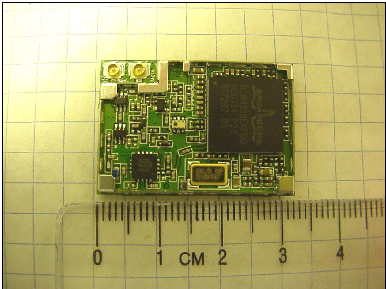
Photograph 14: Top of Radio with Shield Removed
