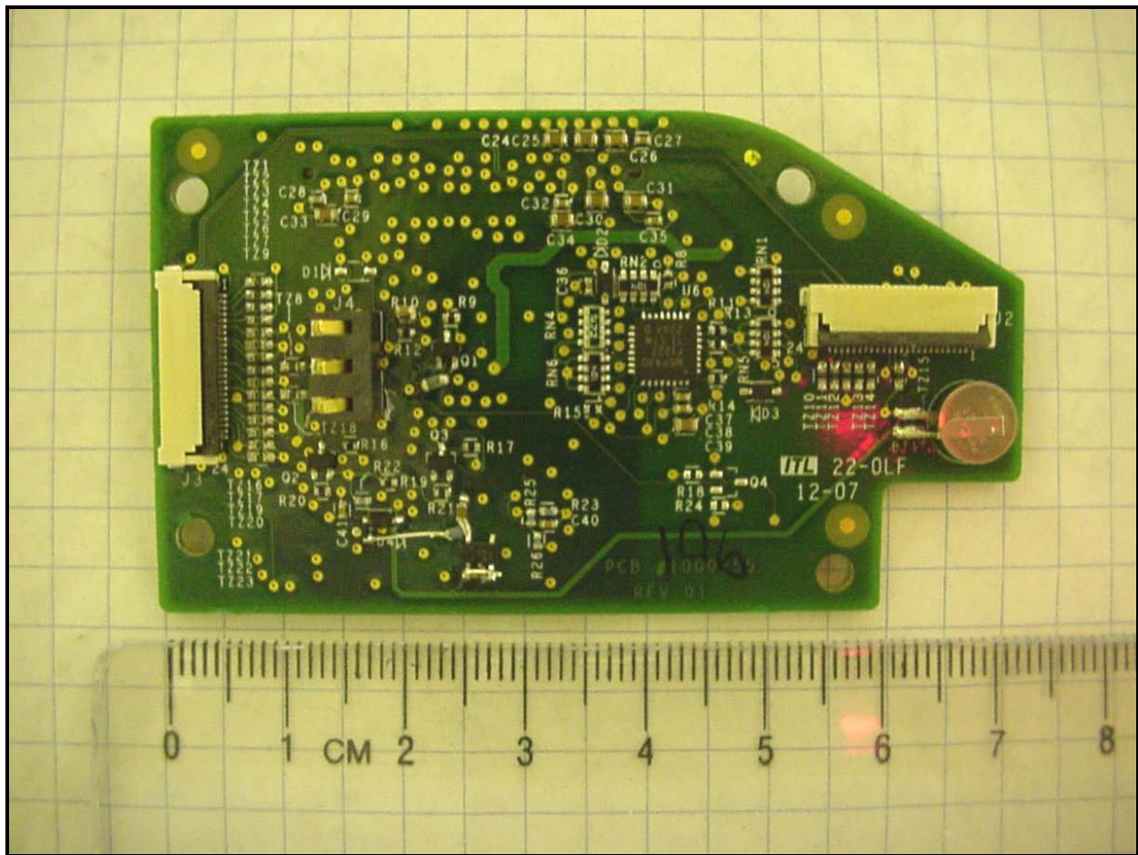
Photograph 6: Bottom PCB Showing Battery Connection
