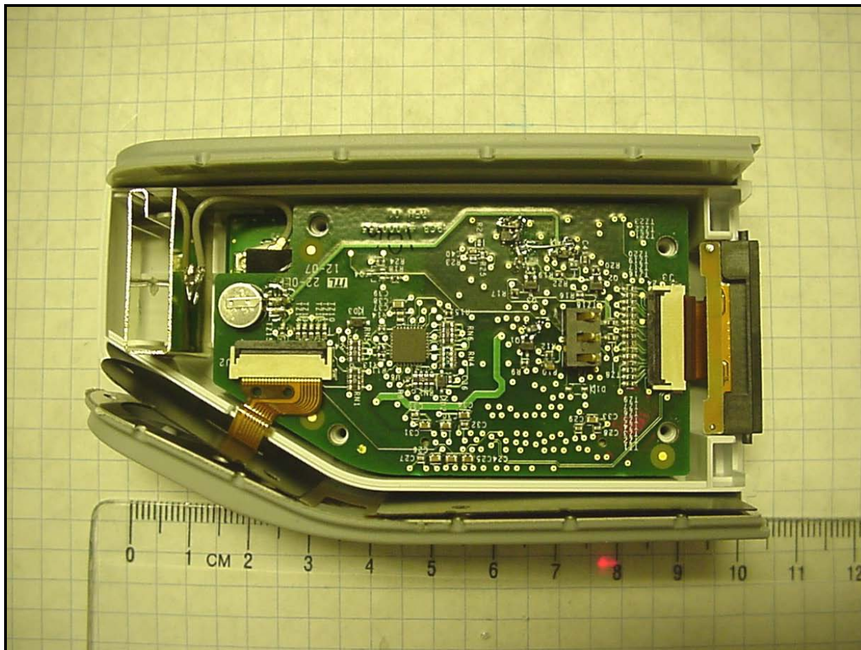
Photograph 5: Bottom PCB in Case
