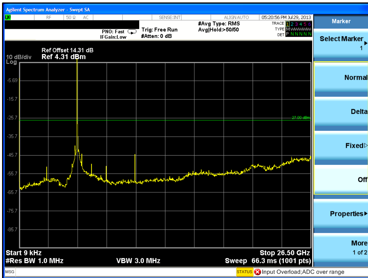
Plot 8-7: Undesirable Emissions Channel 52 (5260 MHz); 9 kHz – 26.5 GHz
