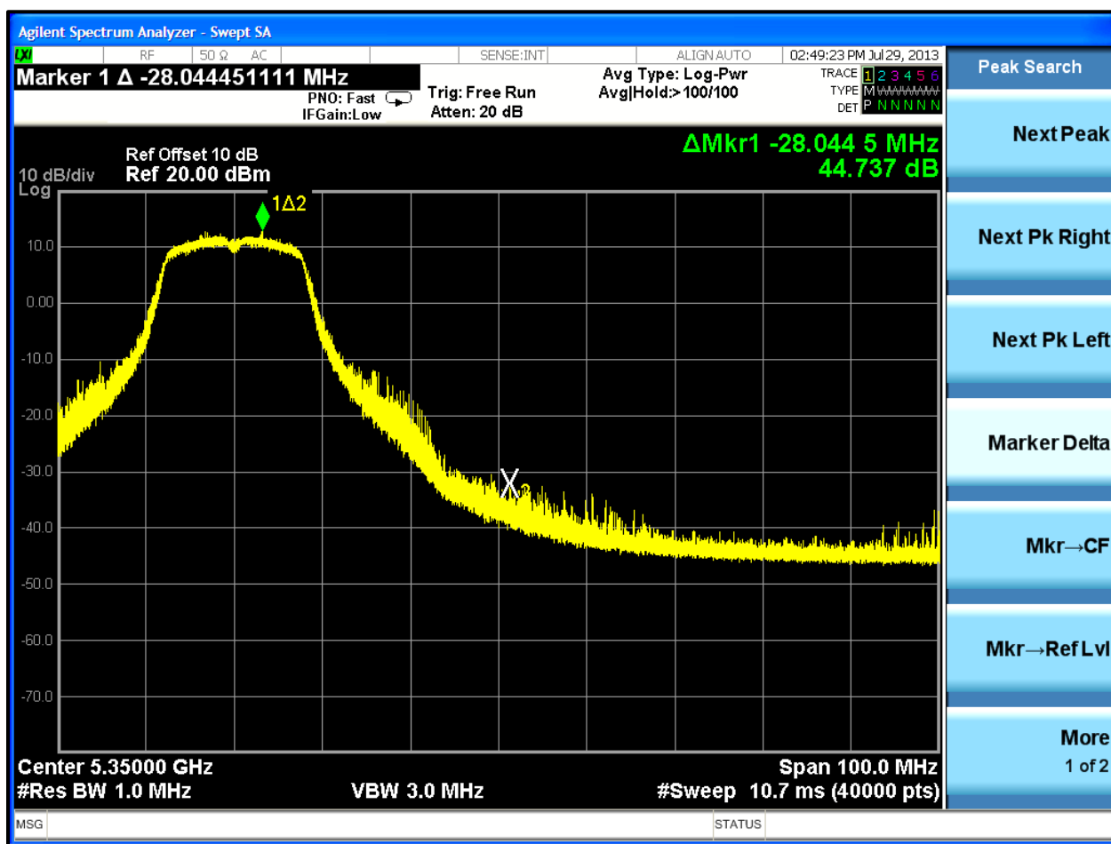
Plot 7-2: Upper Band Edge: Measurement Channel 64 (TX Frequency: 5320 MHz)
