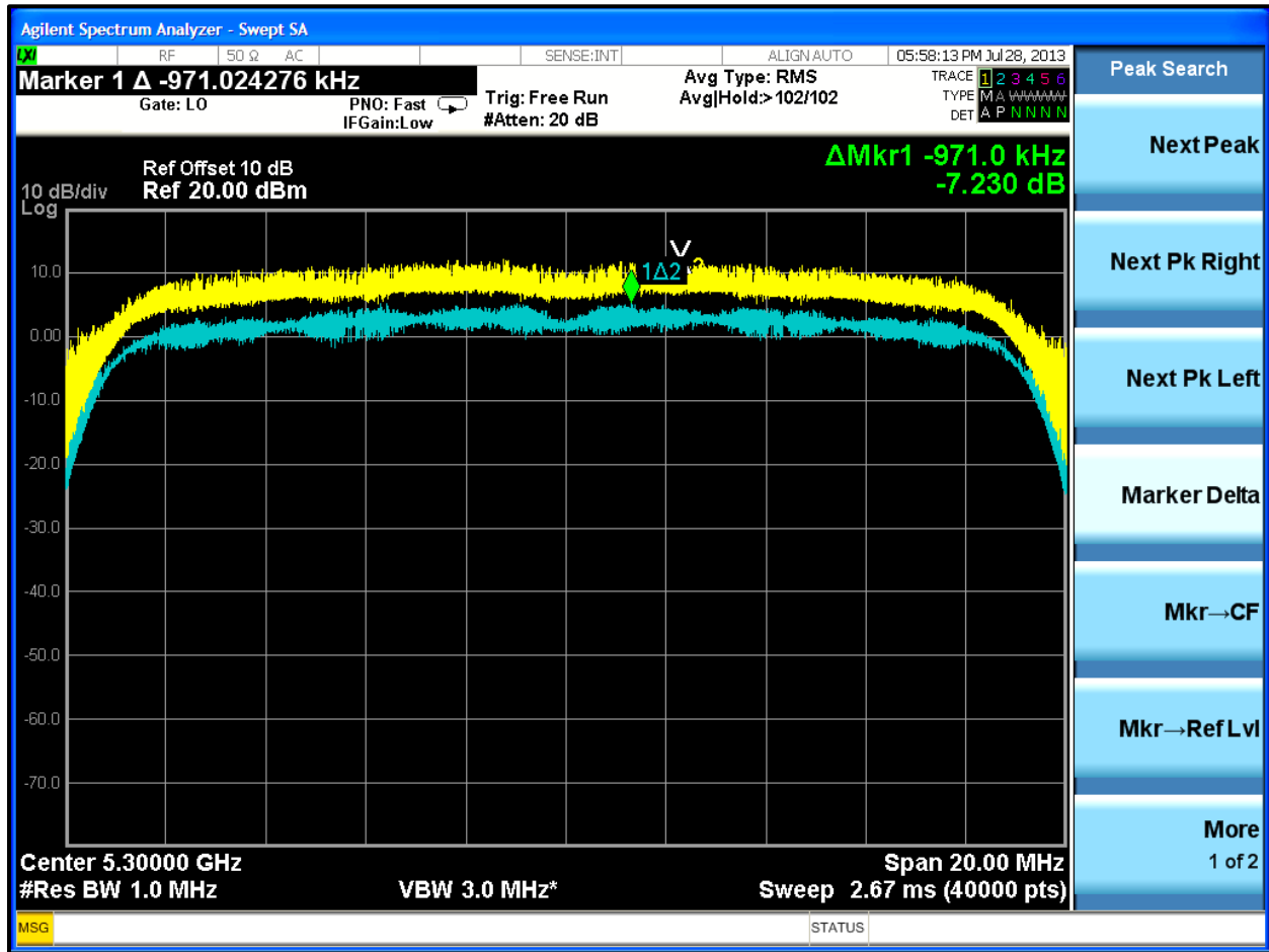
Plot 4-10: Peak Power Excursion: 7.2 mbps
