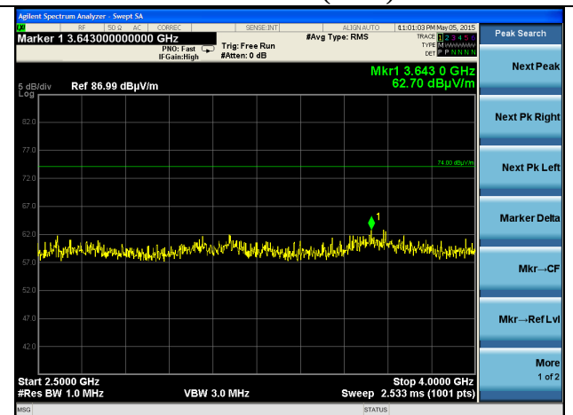
2.5-4 GHz (Peak)
