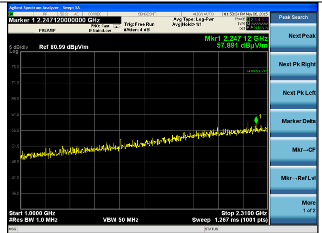
1-2.31 GHz (Peak)
