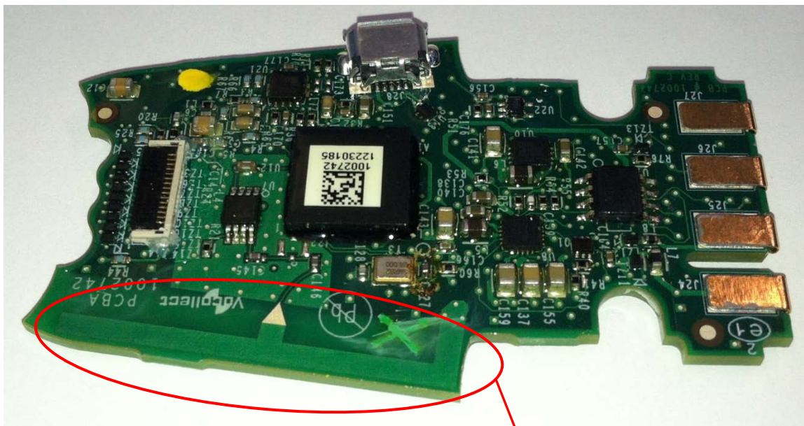
Bluetooth Antenna
