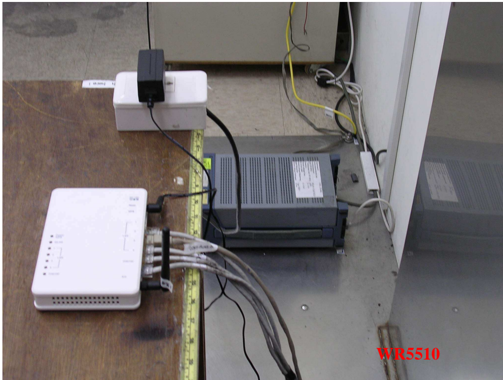
Photo 2: Conducted Emission Test Set-up photo
