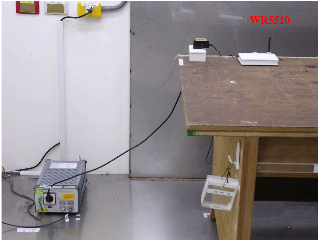
Photo 1: Conducted Emission Test Set-up photo
