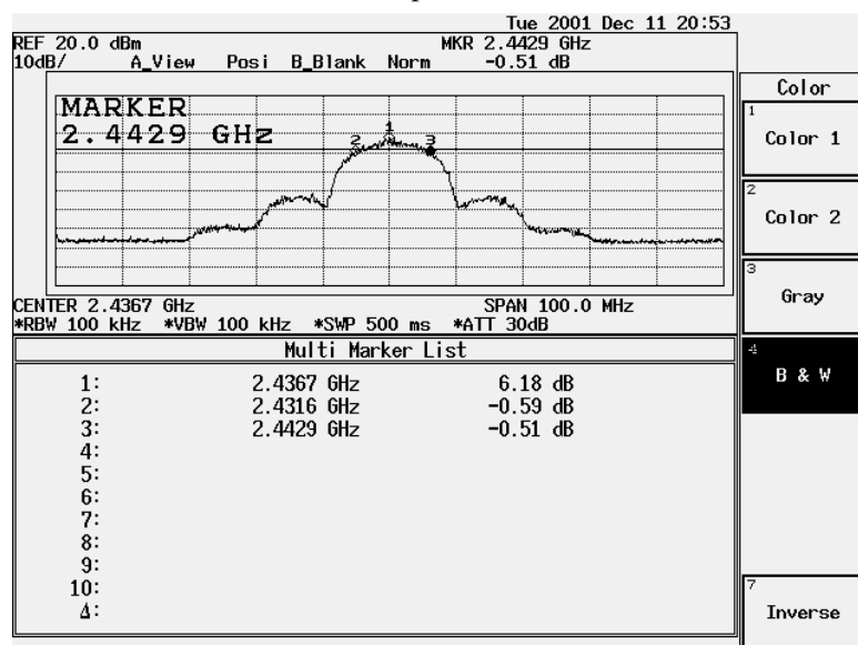
Figure Channel 6: 11Mbps
