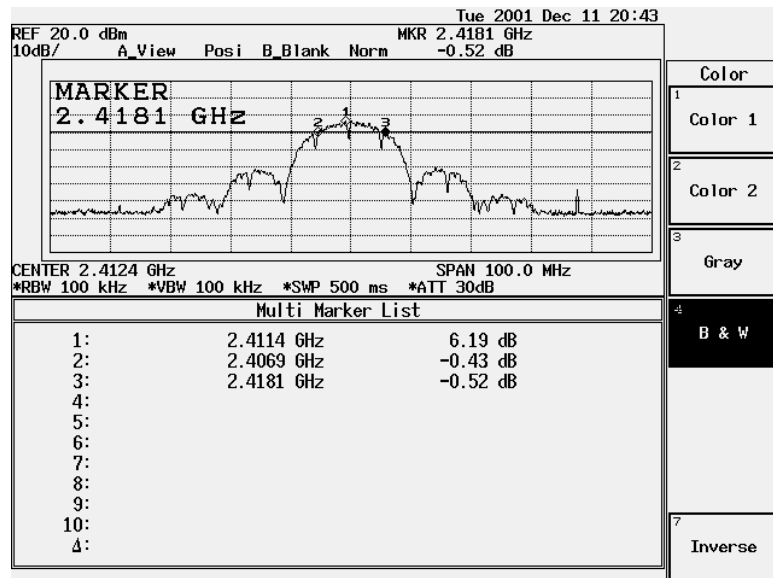
Figure Channel 1: 11Mbps
