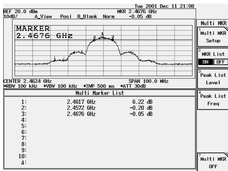
Figure Channel 11: 11Mbps
