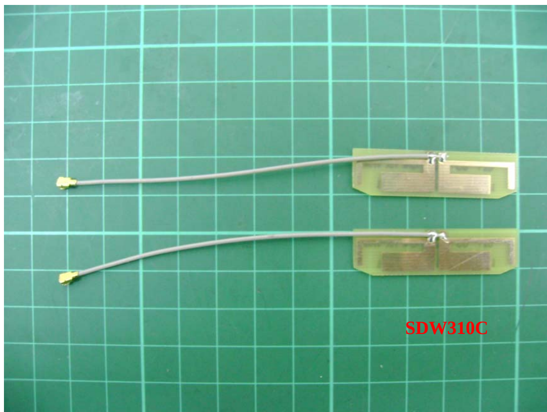
PCB antenna
