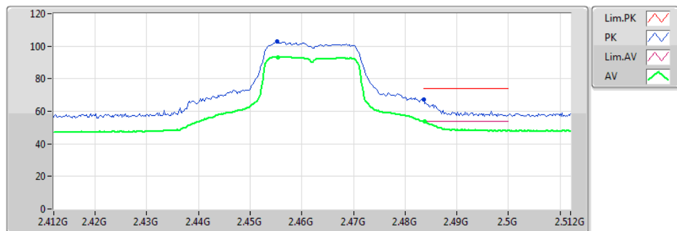
RE above 1GHz;Band:2.4G;HT20;BWch:20MHz;Nss:2,(M8-15);Nant:2;Ch:2462MHz;TX
