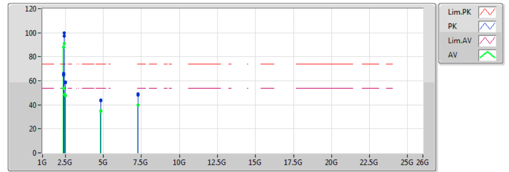
RE above 1GHz;Band:2.4G;HT40;BWch:40MHz;Nss:2,(M8-15);Nant:2;Ch:2422MHz;TX
