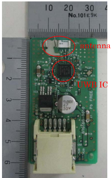
PCB Front View
