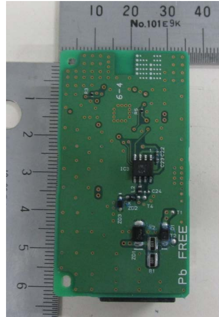
PCB Rear View
