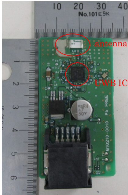
PCB Front View
