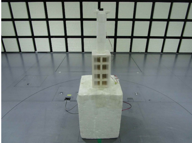
Front (960 MHz to 1000 MHz)
