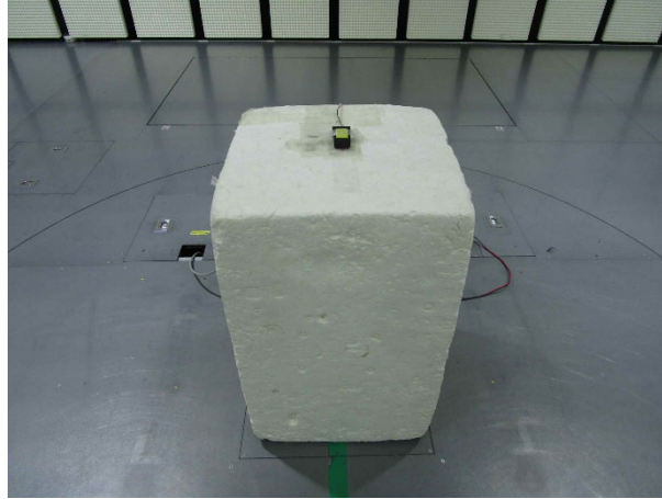
Front (Below 30 MHz)
