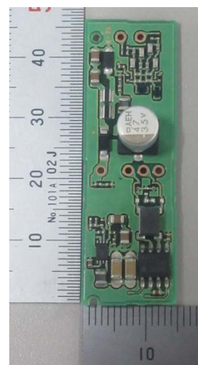
Bottom View
