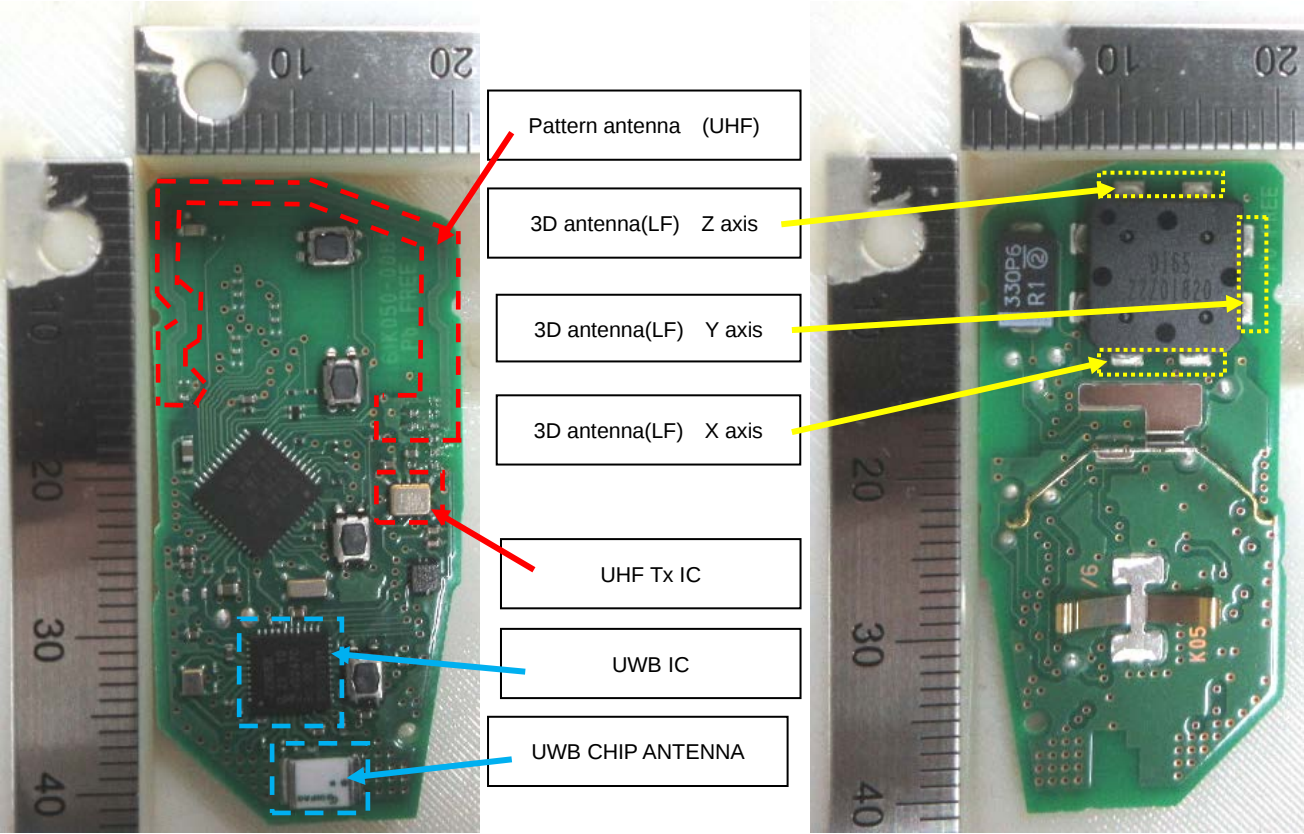
Antenna position
