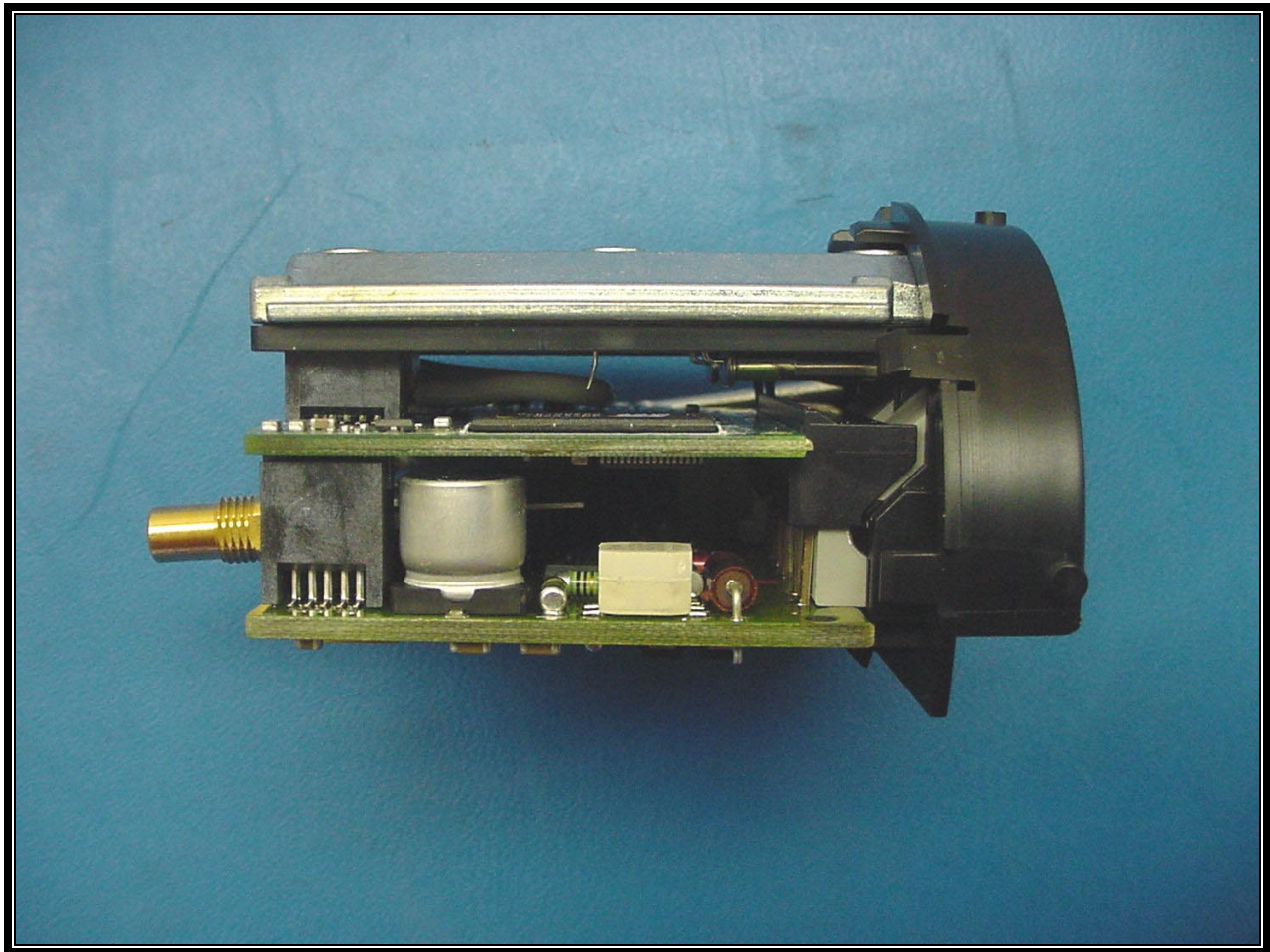
PHOTOGRAPH 28: EUT MODULE PARTS SIDE VIEW
