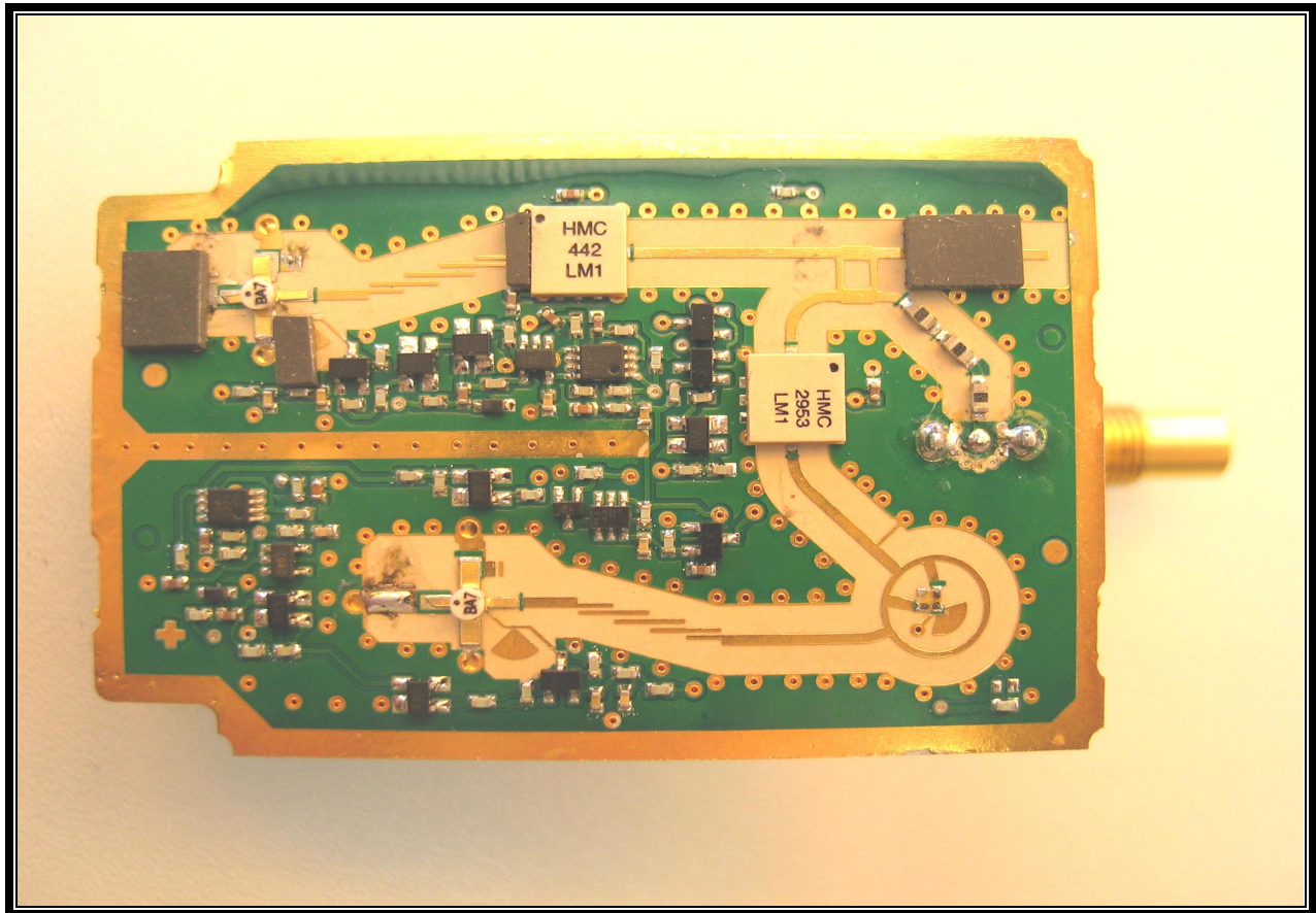
PHOTOGRAPH 36: EUT MODULE RF PCB WITH PORT TOP VIEW
