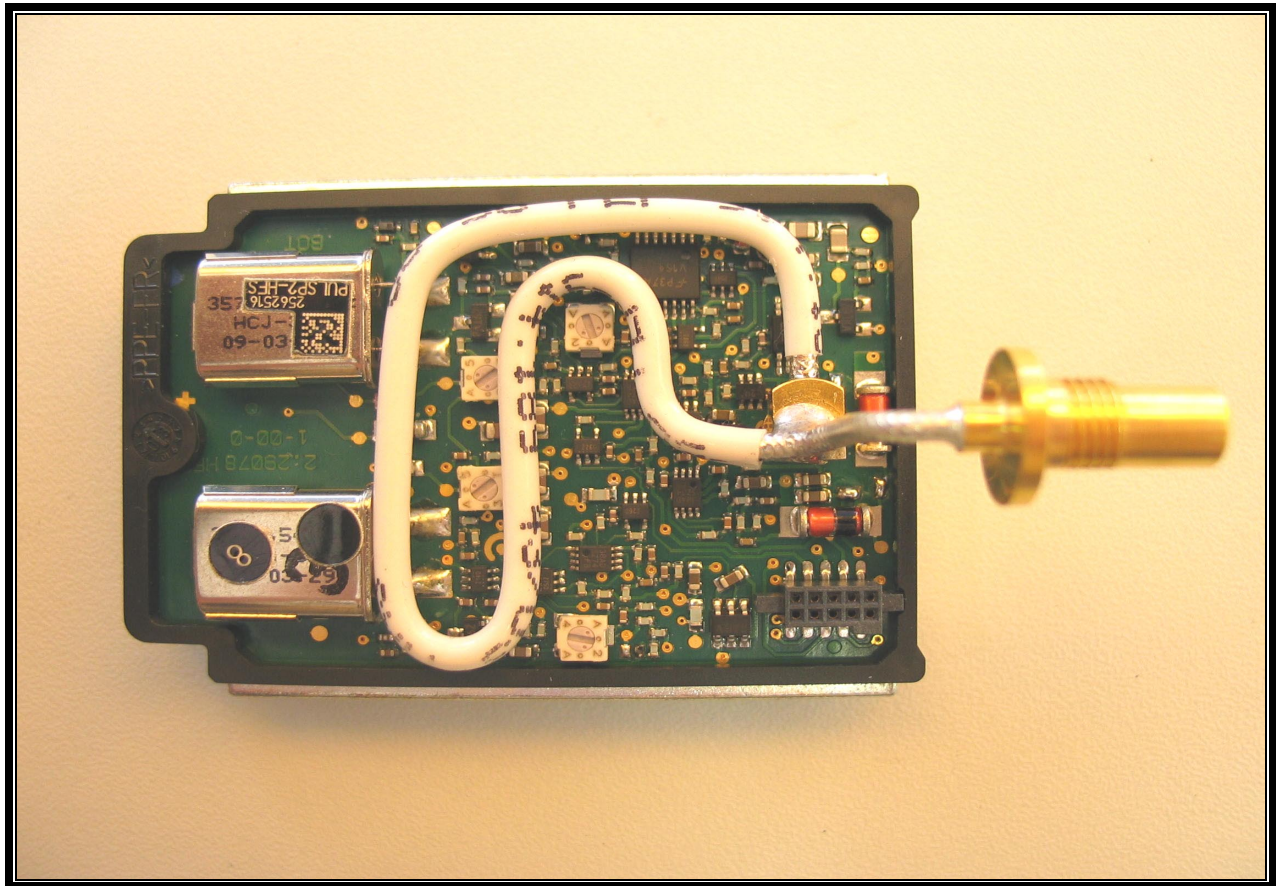
PHOTOGRAPH 37: EUT MODULE RF PCB WITHOUT PORT BOTTOM VIEW
