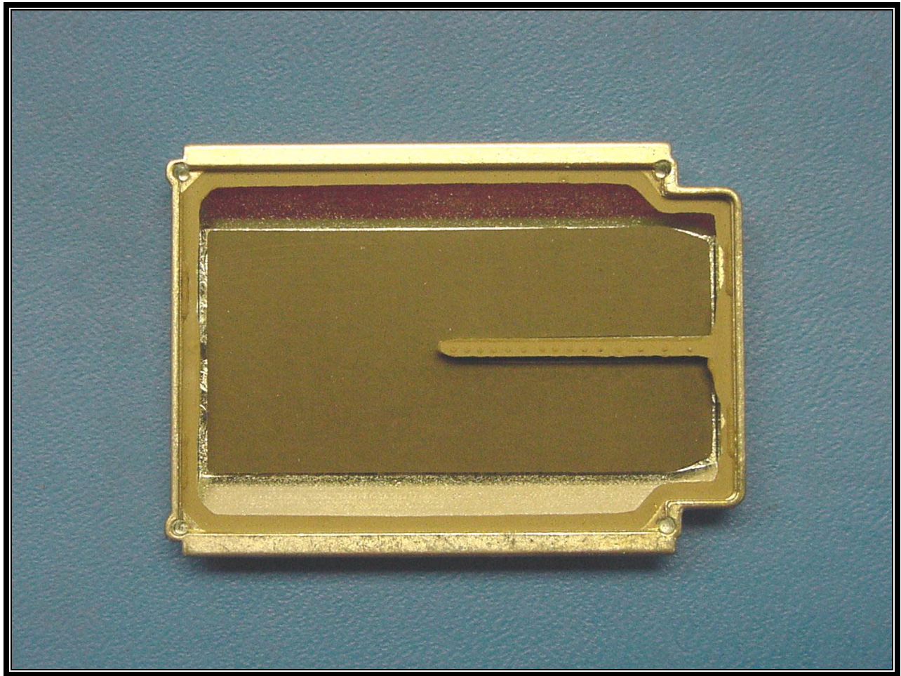
PHOTOGRAPH 34: EUT MODULE RF PCB SHIELD TOP VIEW
