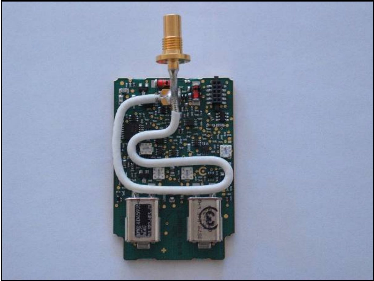
Photograph 17: Microwave Board (Component Side)
