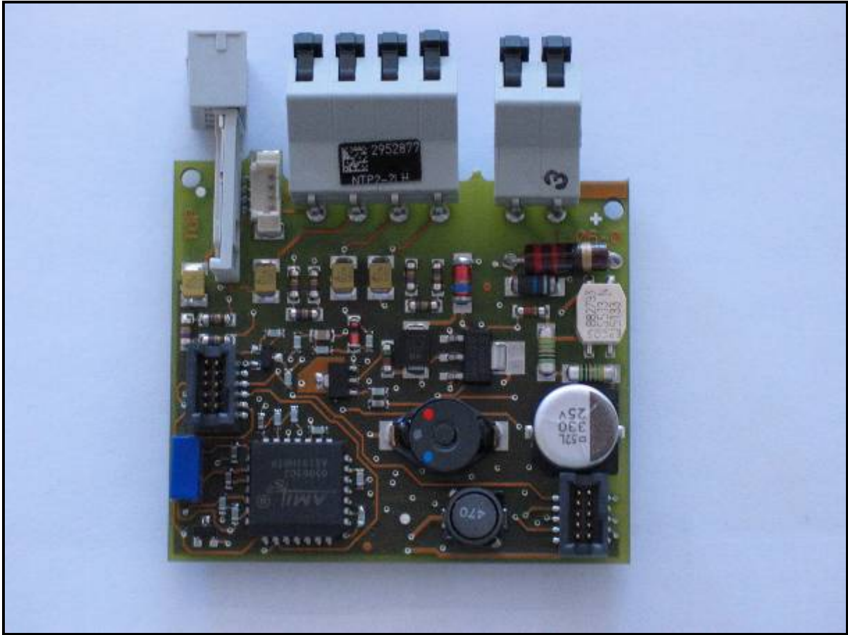
Photograph 12: Power Supply Board (Component Side)
