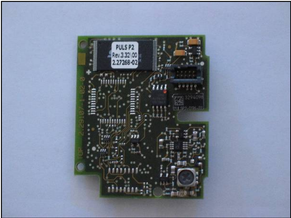
Photograph 14: CPU Board (Solder Side)
