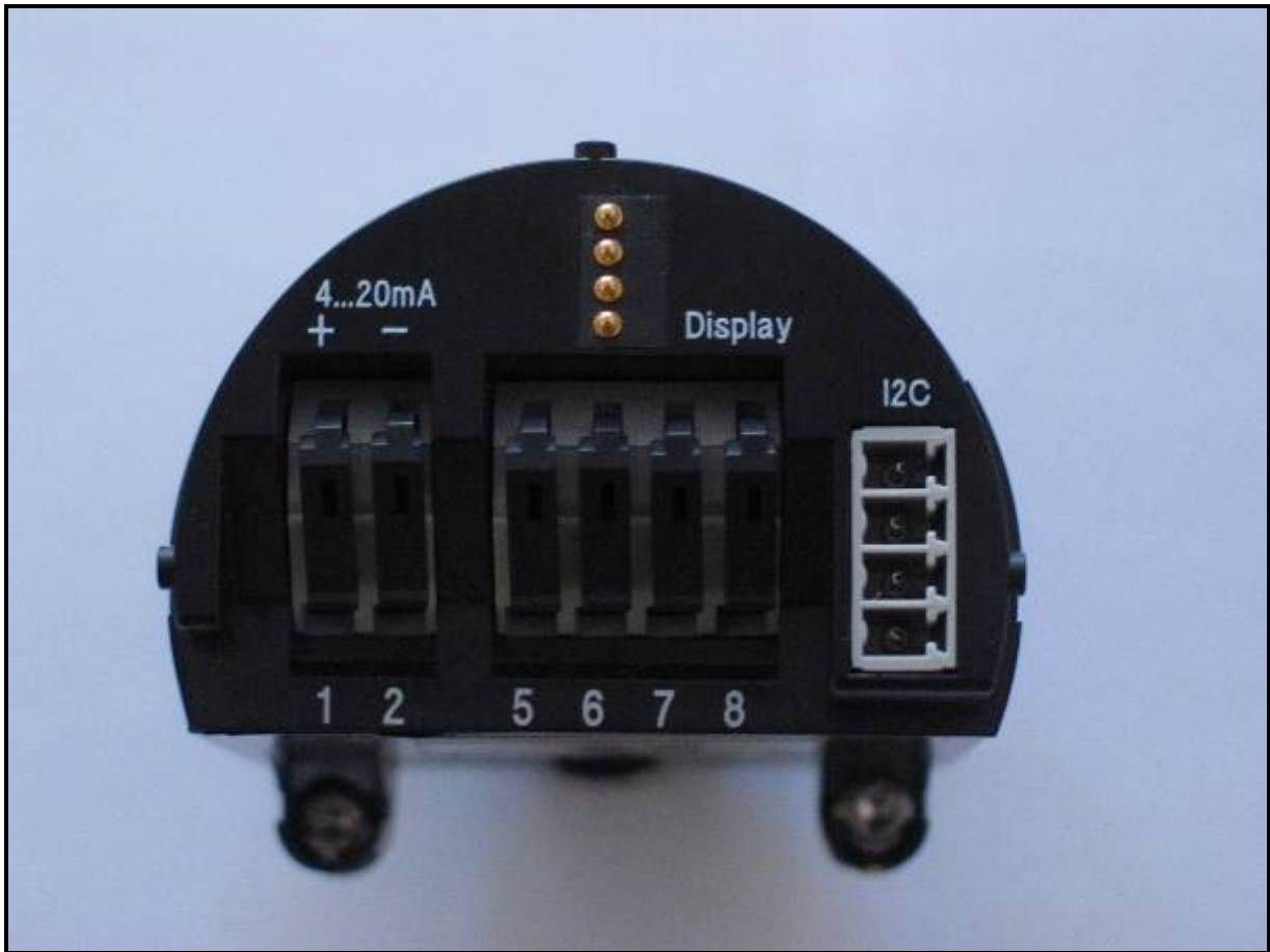
Photograph 20: Electronics Can (Top Side)
