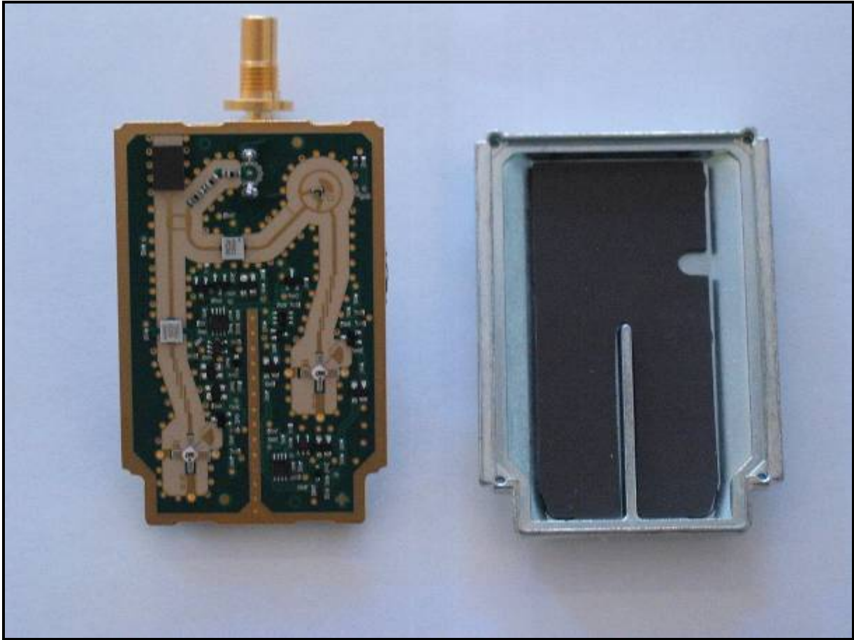
Photograph 16: Microwave Board (Solder Side) + Shielding
