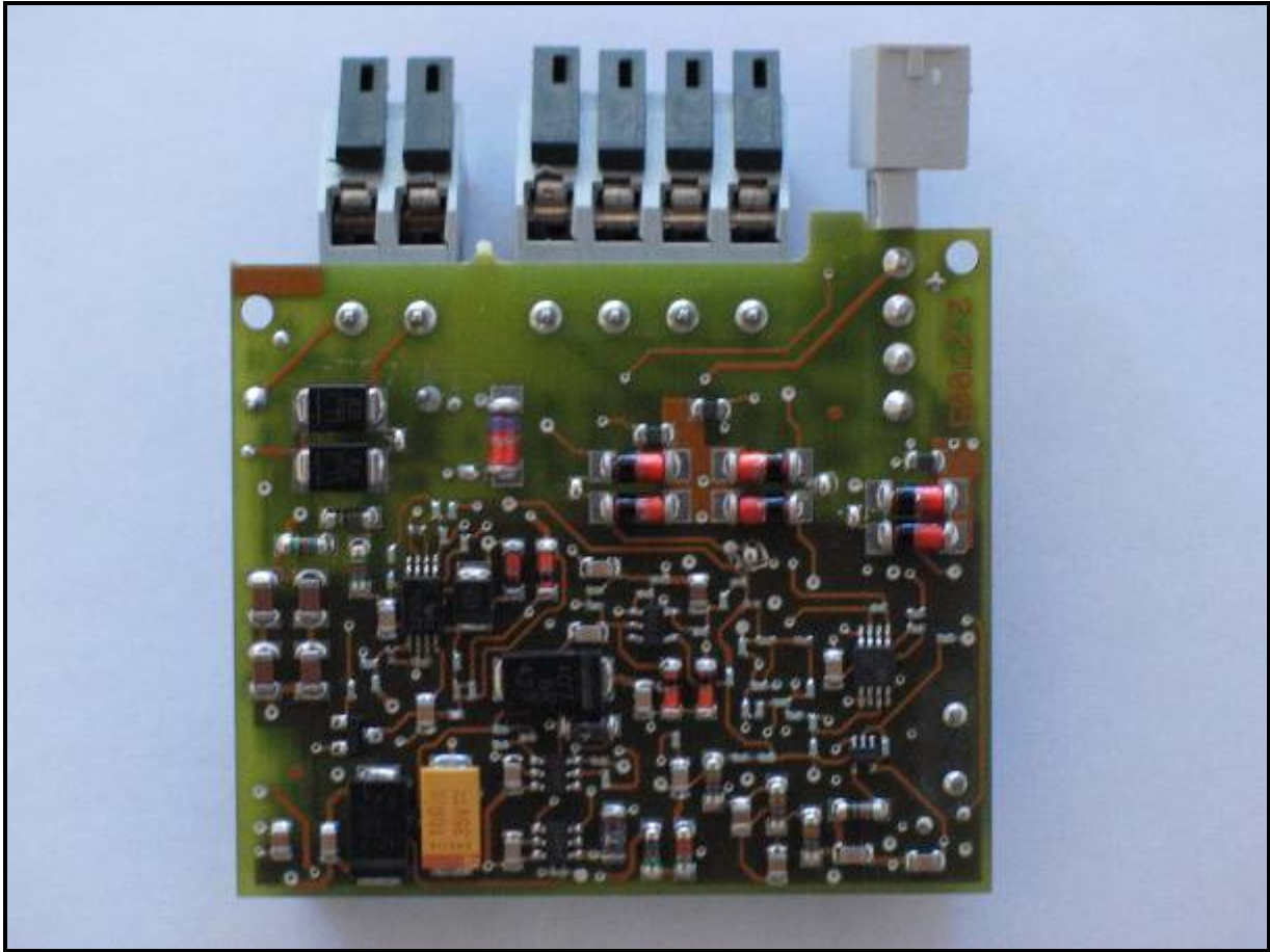
Photograph 13: Power Supply Board (Solder Side)
