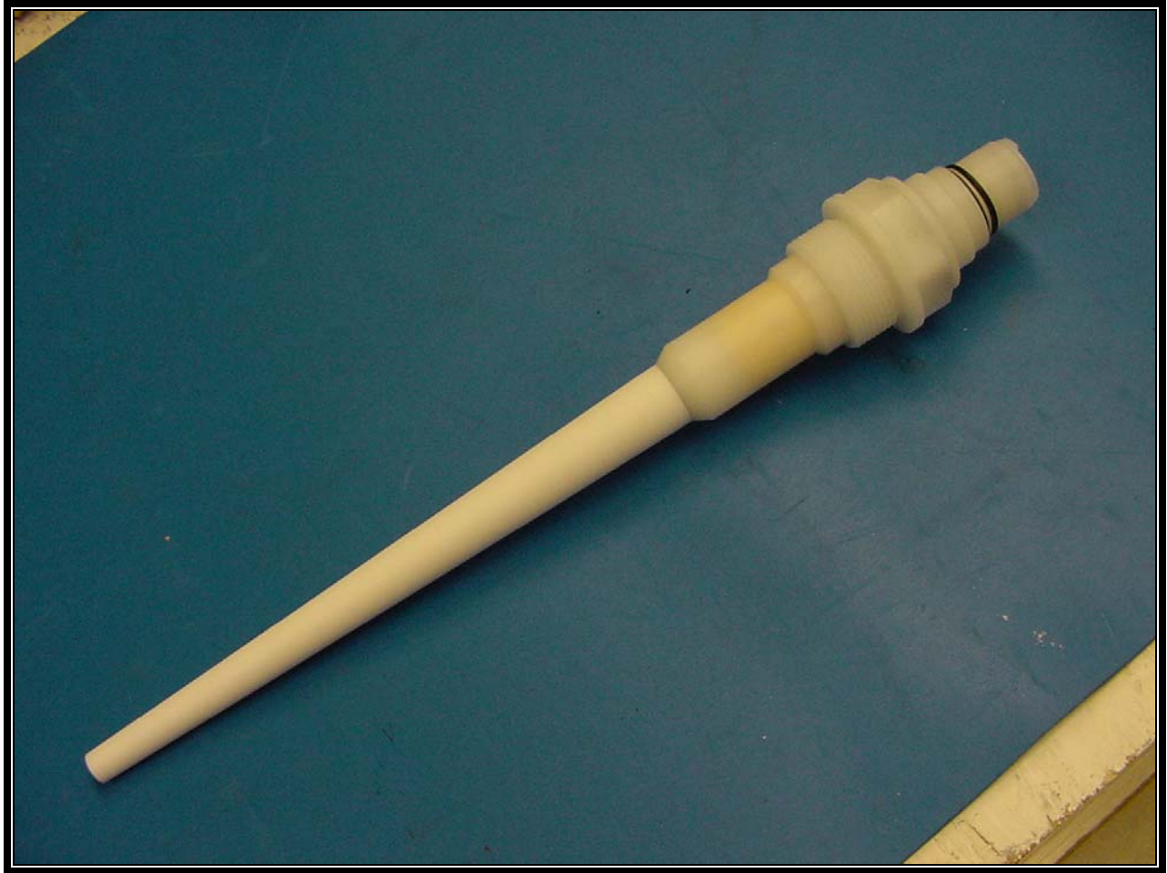
PHOTOGRAPH 20: EUT 17 DBI ROD ANTENNA
