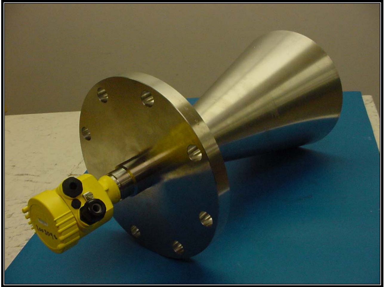
PHOTOGRAPH 23: EUT WITH 21.0 DBI HORN ANTENNA
