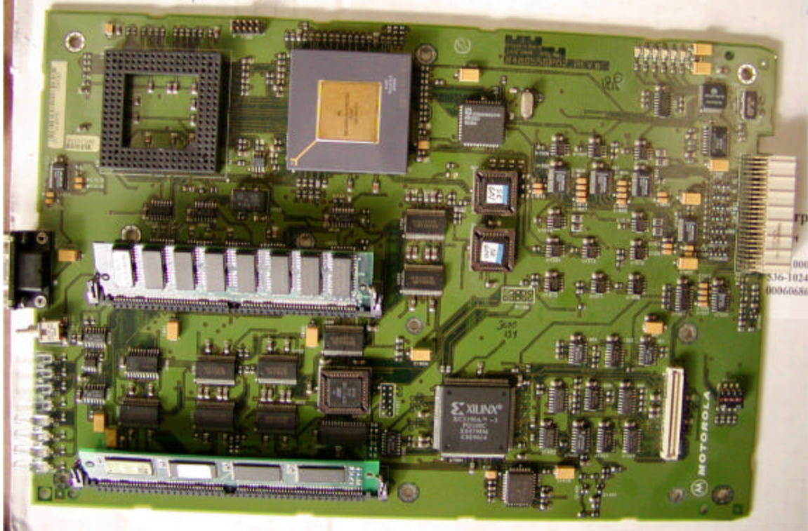
RF BATON OCM (top view)
