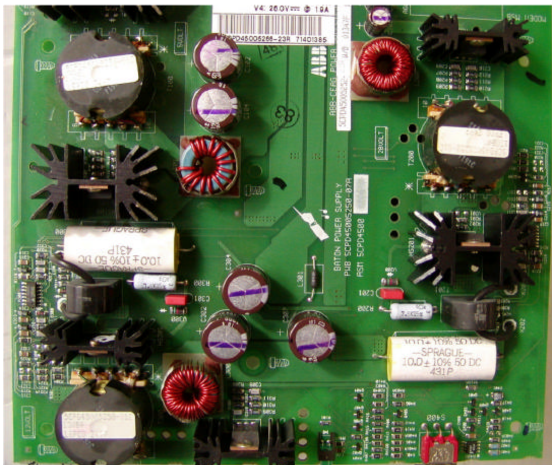
RFO-DC/DC converter part1.2(topview)
