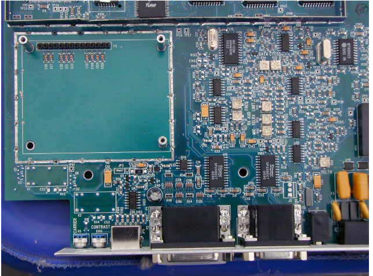
Main board bottom left corner
