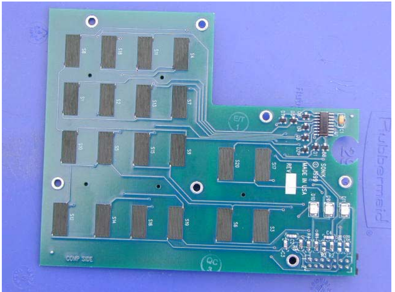
Keypad board front
