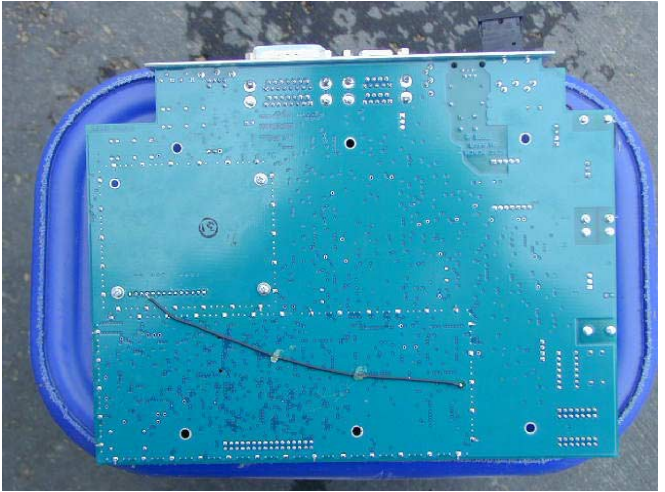
Main board back
