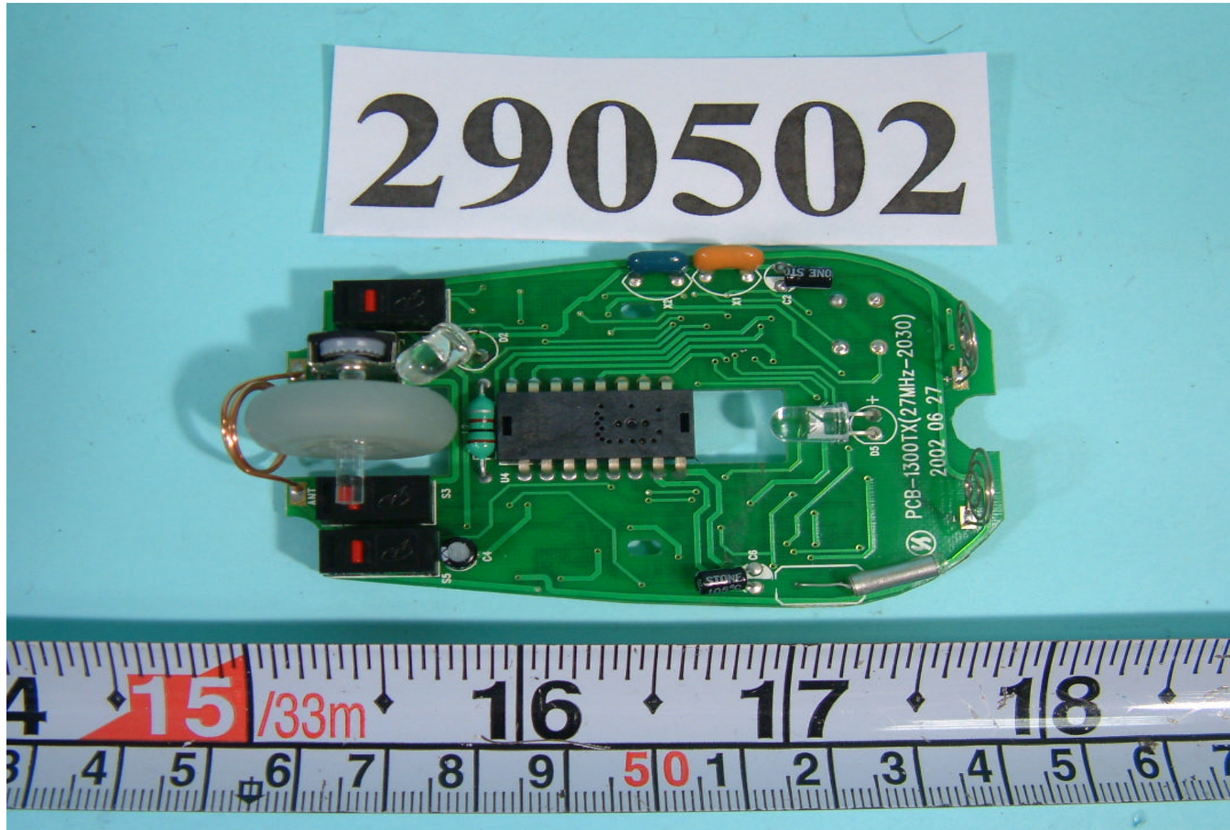
Front side of Main Board(MOUSE)
