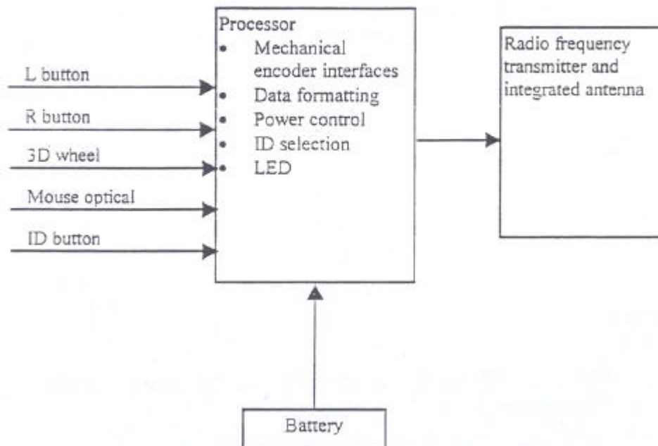
Figure 2. Mouse Unit Block Diagram
