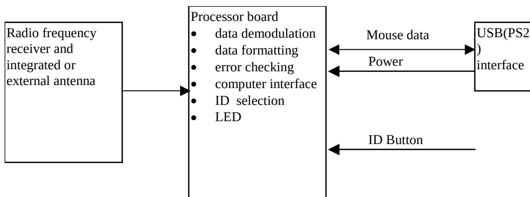
Figure 2. Mouse Unit Block Diagram
