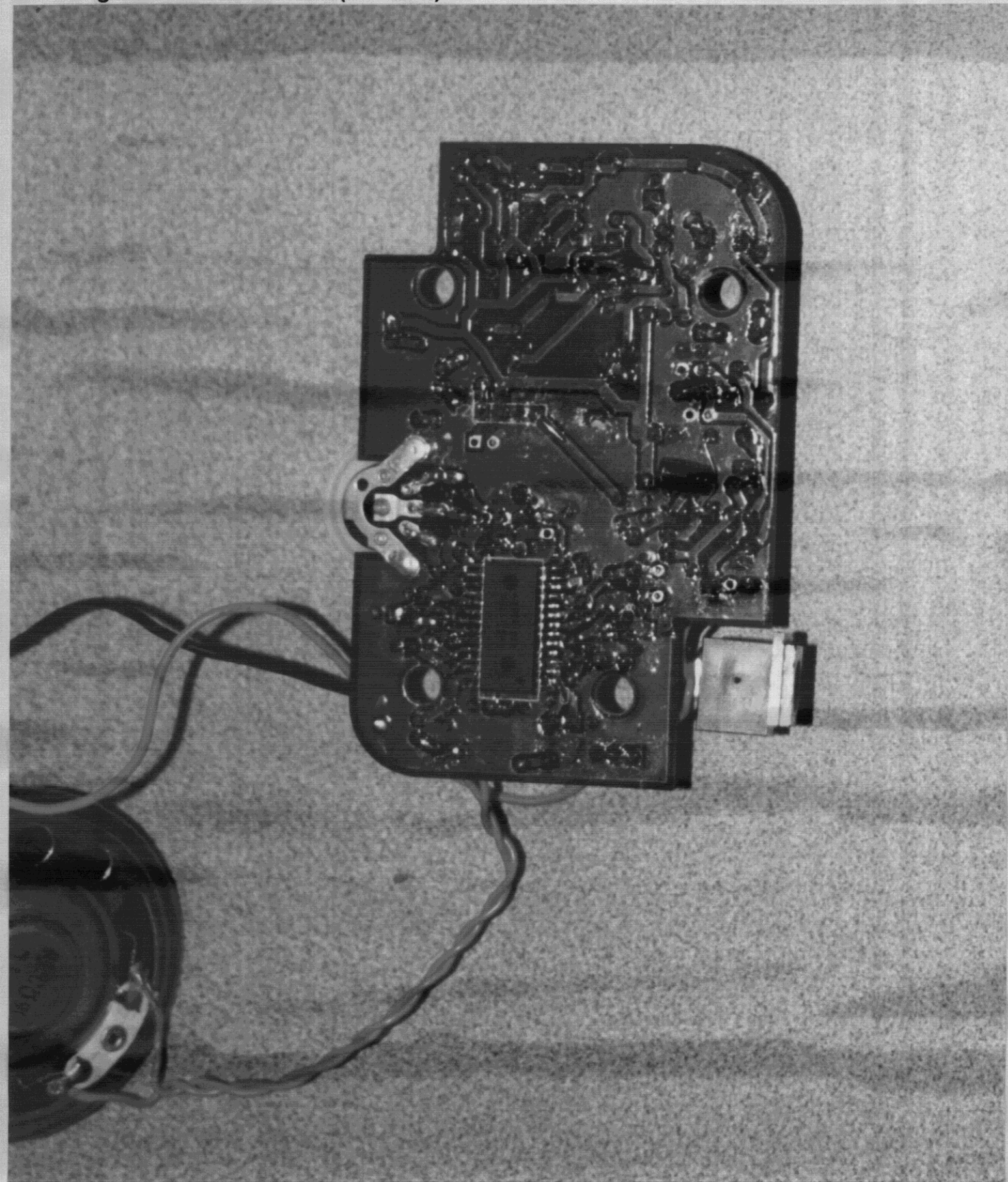
Figure 4.7 Controller PCB (Foil Side)
