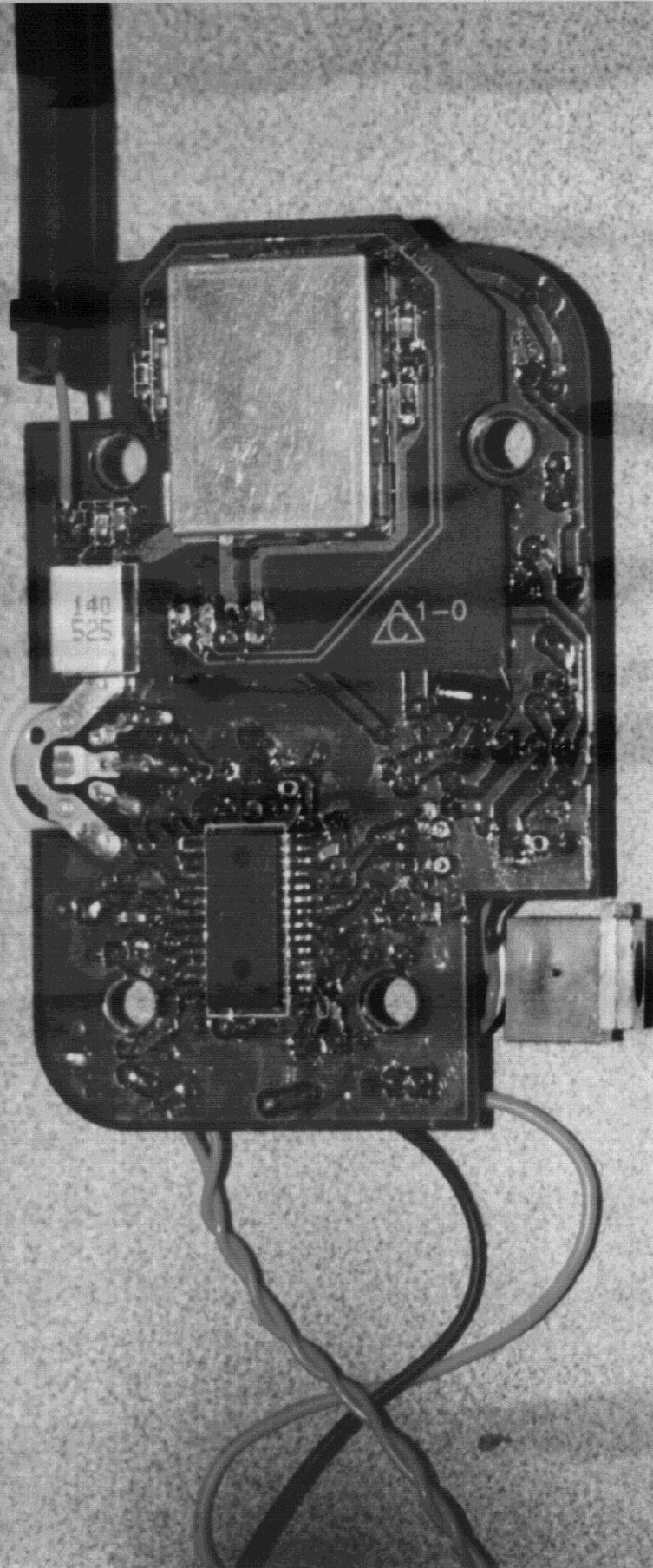
Figure 4.5 RF & Controller PCB Assembled
