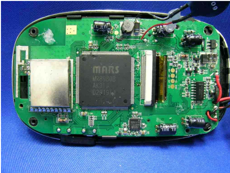
Parent Unit Main PCB front side (View 2)
