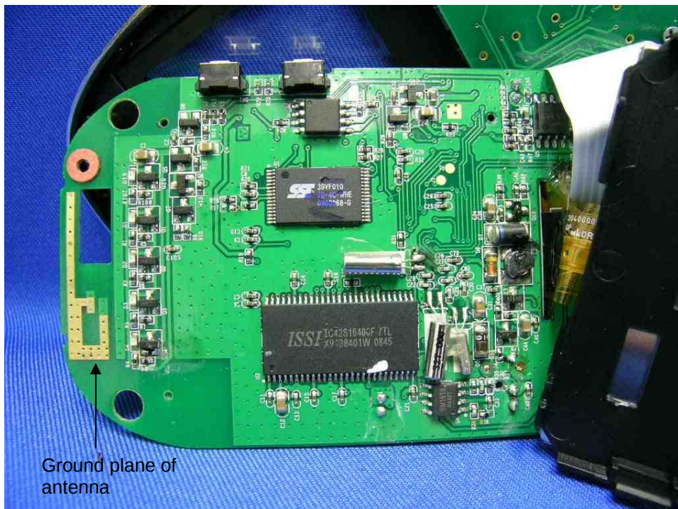
Parent Unit Main PCB rear side (View 1)
