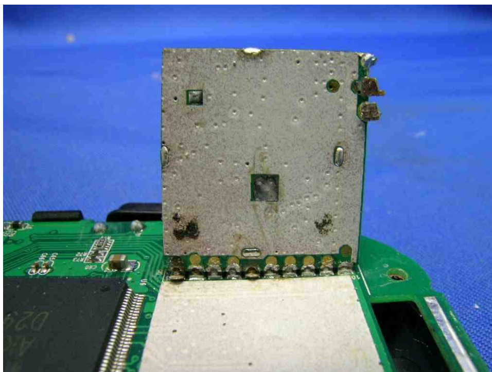
Parent Unit RF Module PCB rear side
