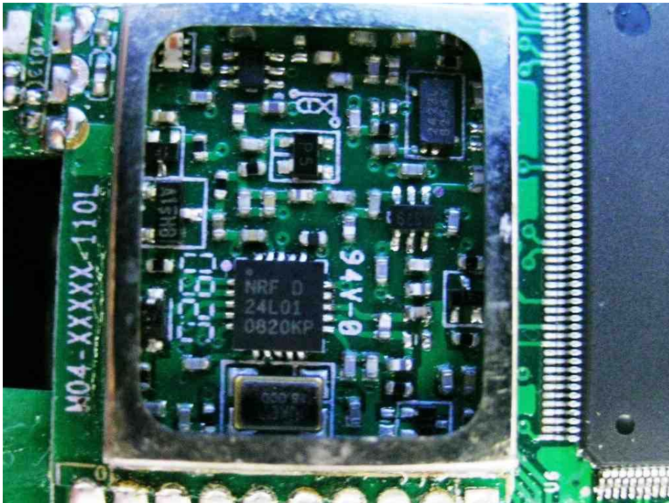
Parent Unit RF Module PCB front side
