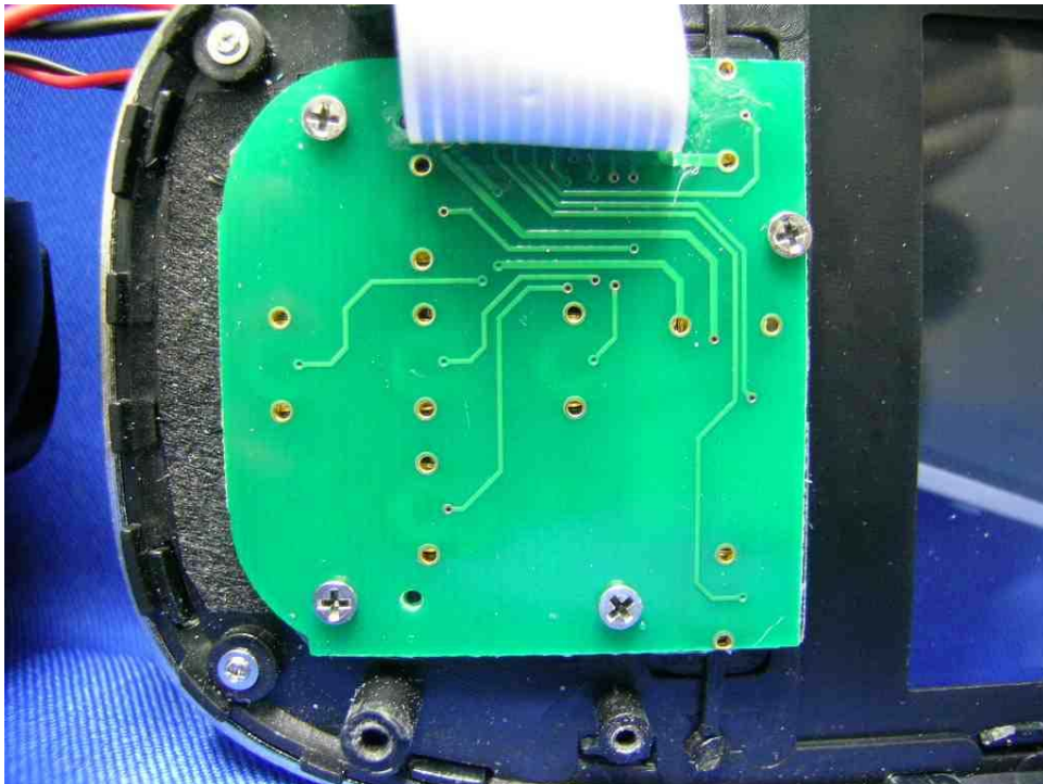
Parent Unit Keypad PCB rear side (View 1)
