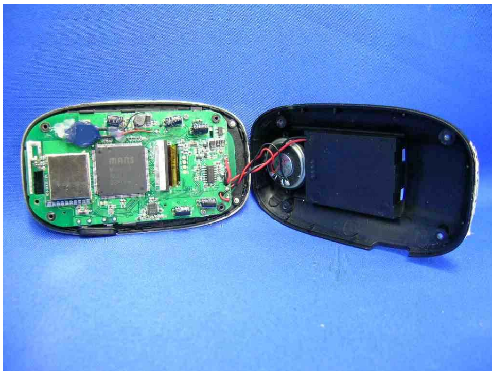
Parent Unit assembly (View 1)
