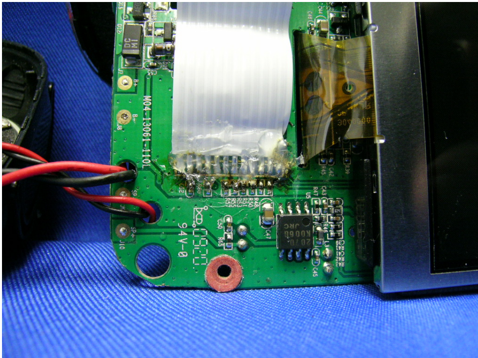
Parent Unit Main PCB rear side (View 3)
