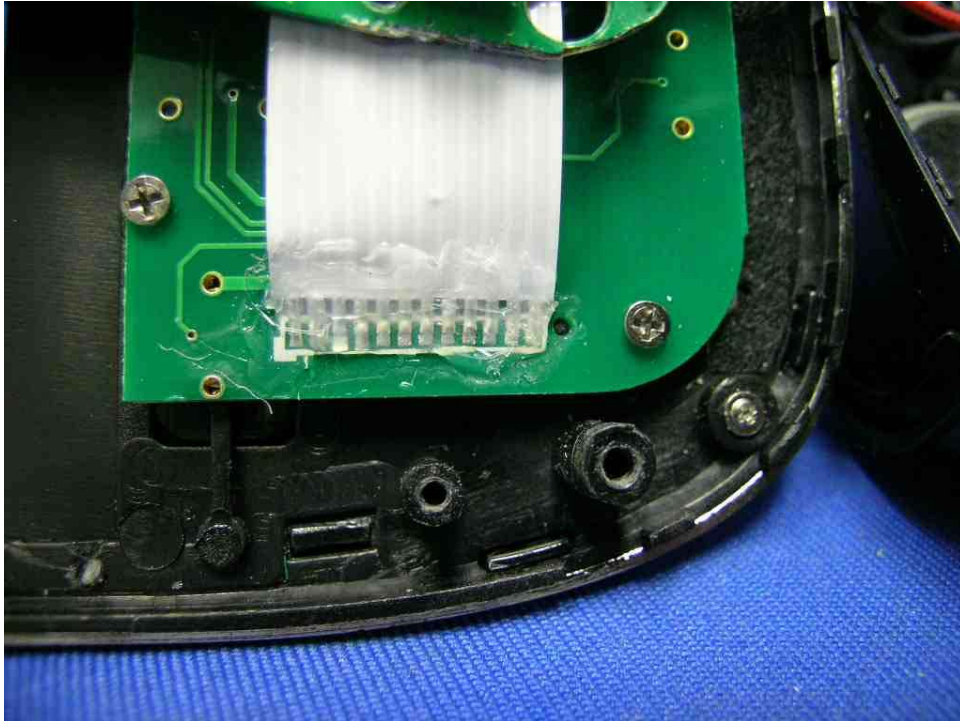
Parent Unit Keypad PCB rear side (View 2)
