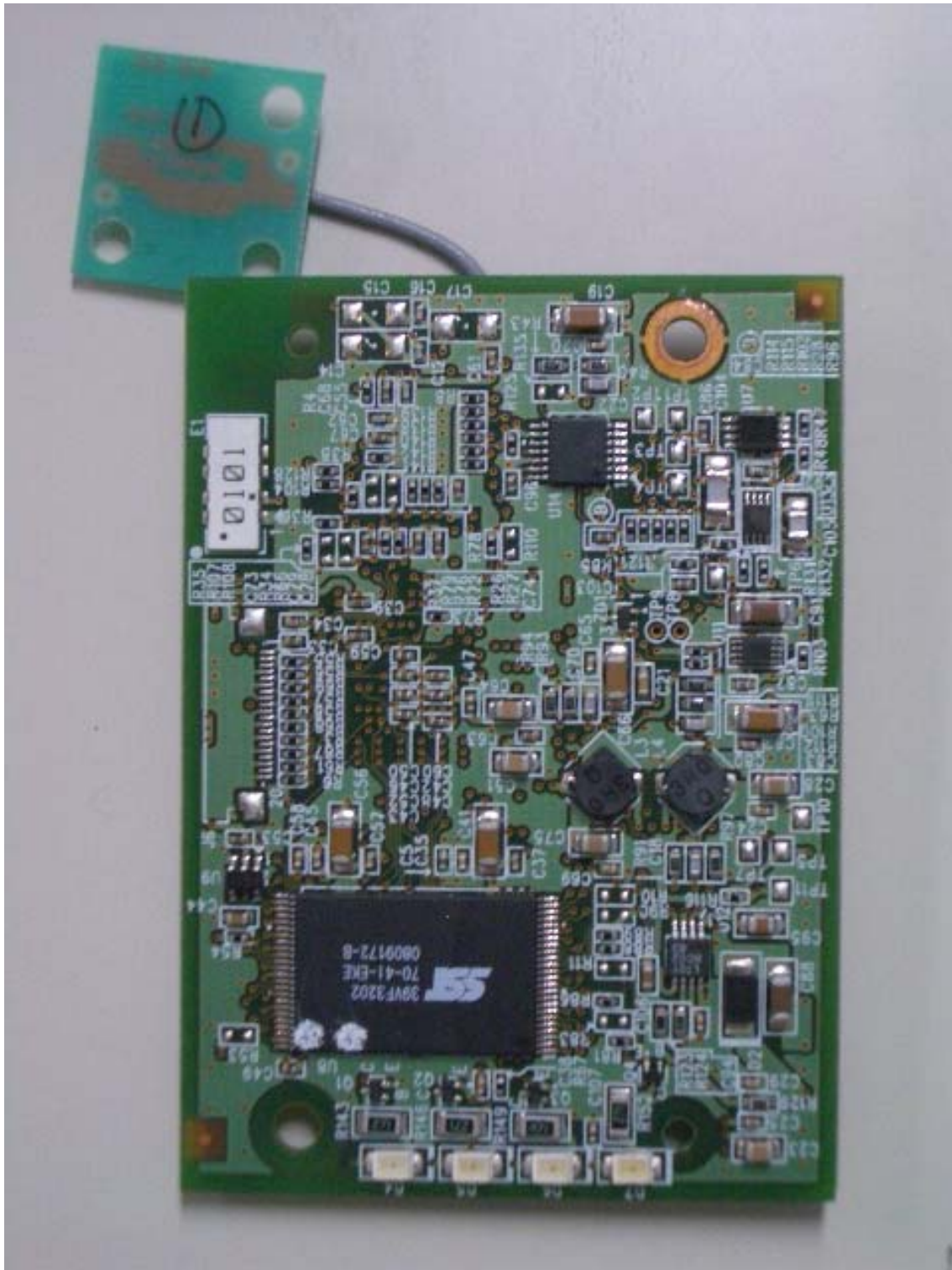
WLAN2USB (Bottom)
