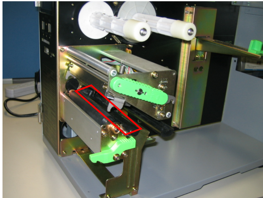
Antenna Holder Position (Side view)
