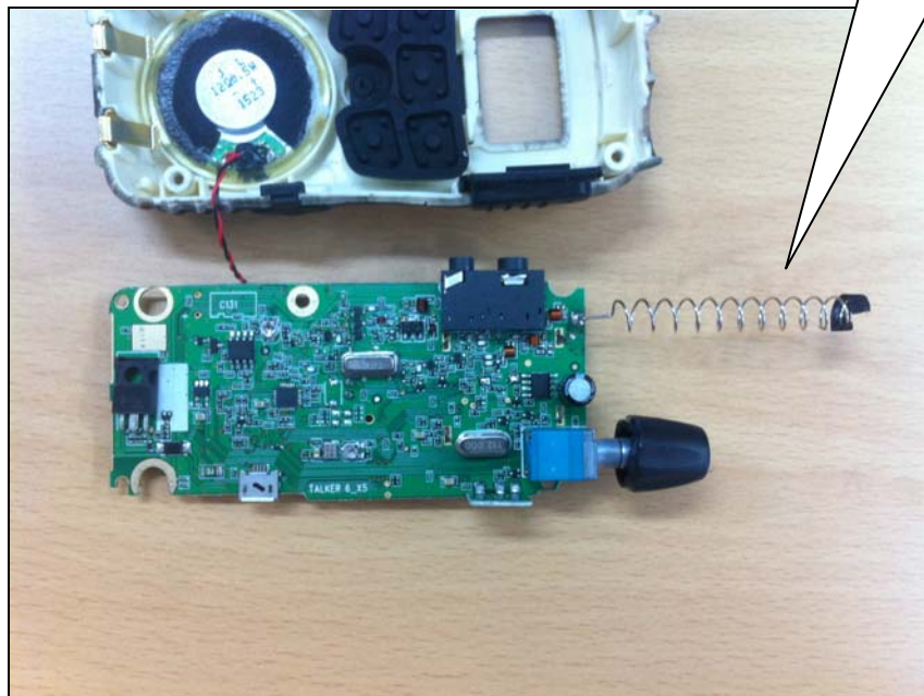
Helical Antenna
