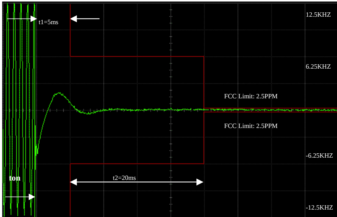
2 Watts, 162.025MHZ 12.5KHZ KEY-UP ATTACK TIME
