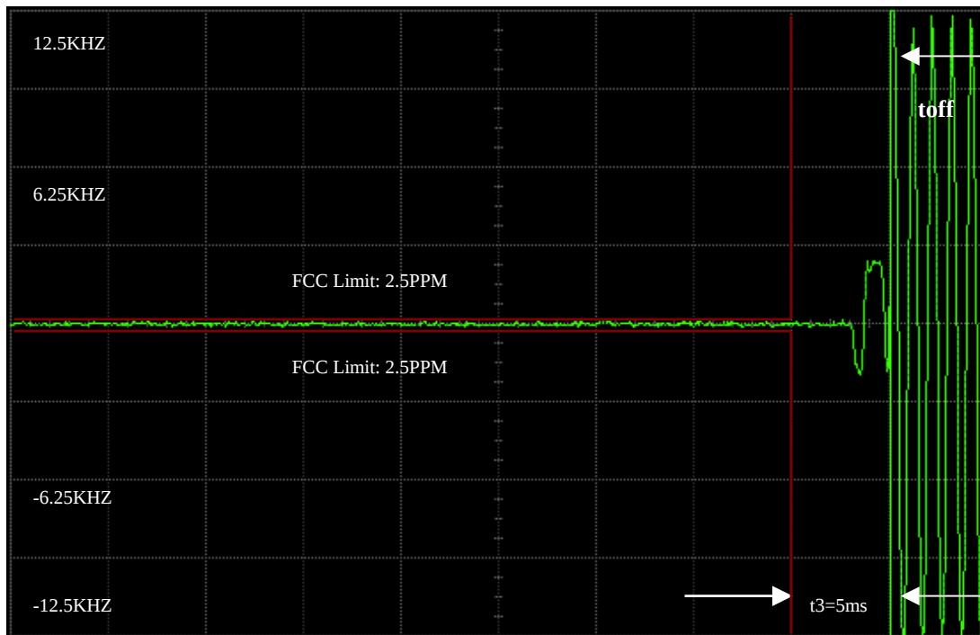
2 Watts, 162.025MHZ 12.5KHZ DE-KEY DECAY TIME
