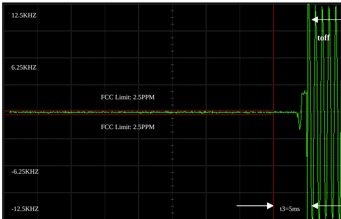
2 Watts, 173.975MHZ 12.5KHZ DE-KEY DECAY TIME
