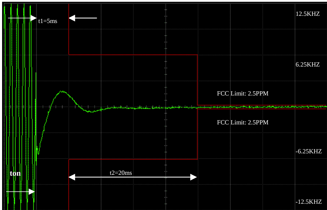
2 Watts, 173.975MHZ 12.5KHZ KEY-UP ATTACK TIME
