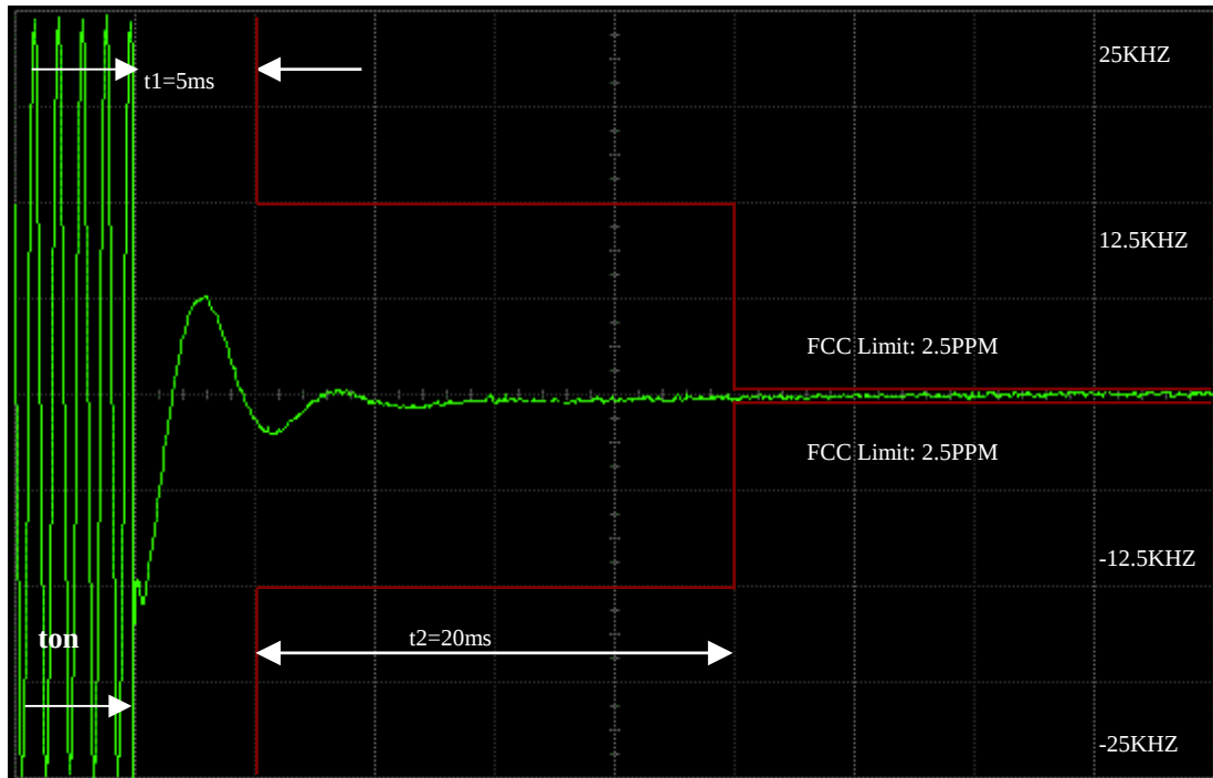
2 Watts, 148.025Mhz 25KHZ KEY-UP ATTACK TIME
