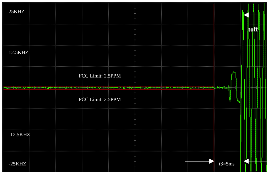
2 Watts, 148.025Mhz 25KHZ DE-KEY DECAY TIME
