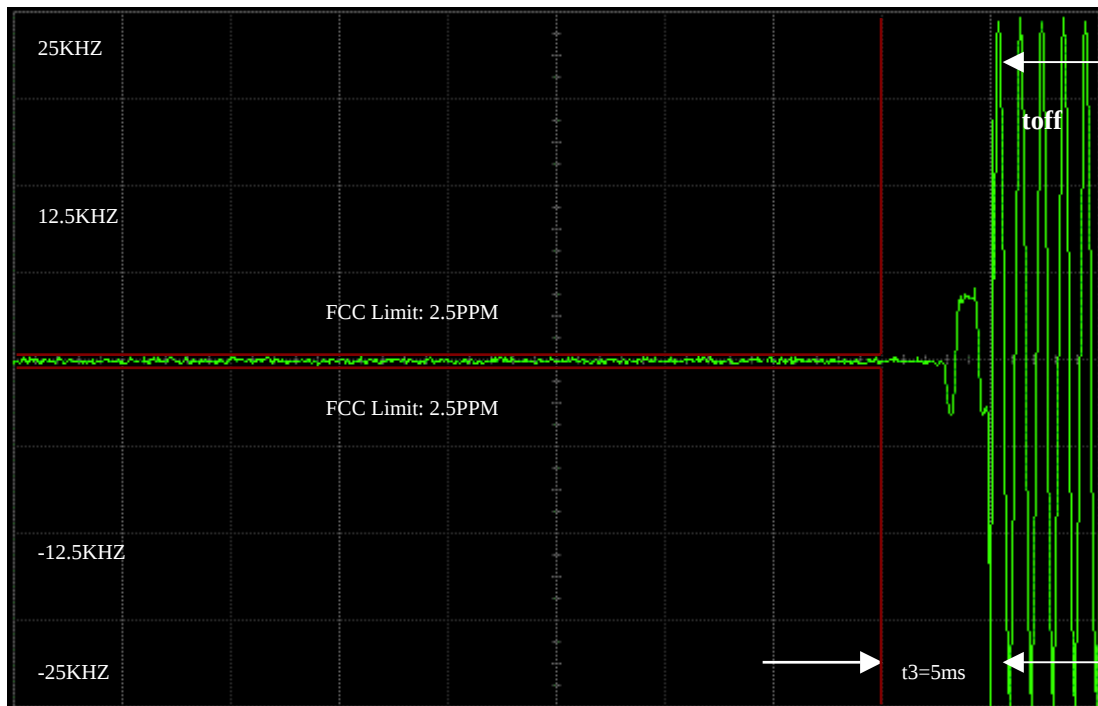
2 Watts, 162.025MHZ 25KHZ DE-KEY DECAY TIME
