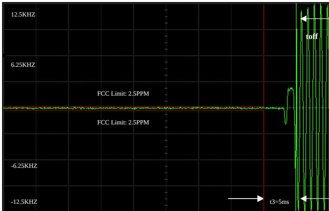
2 Watts, 162.025MHZ 12.5KHZ DE-KEY DECAY TIME
