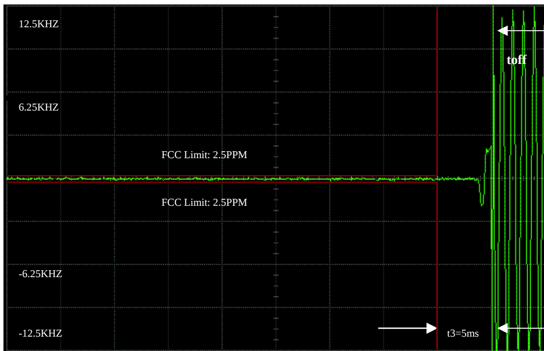
2 Watts, 148.025Mhz 12.5KHZ DE-KEY DECAY TIME
