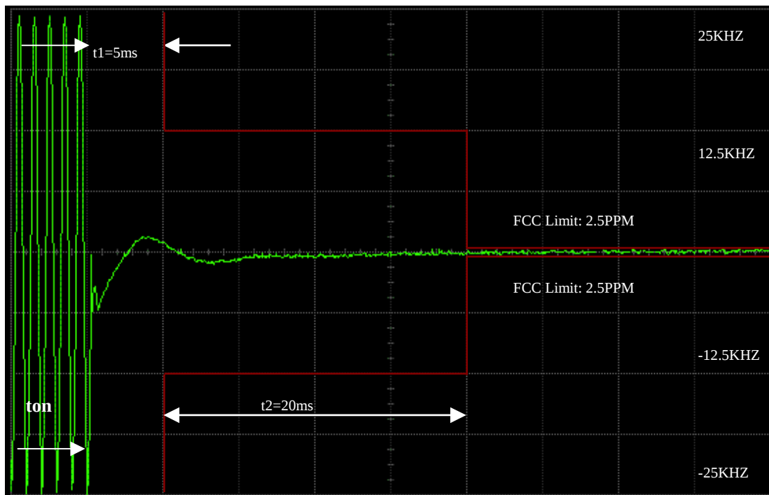
2 Watts, 162.025MHZ 25KHZ KEY UP ATTACK TIME
