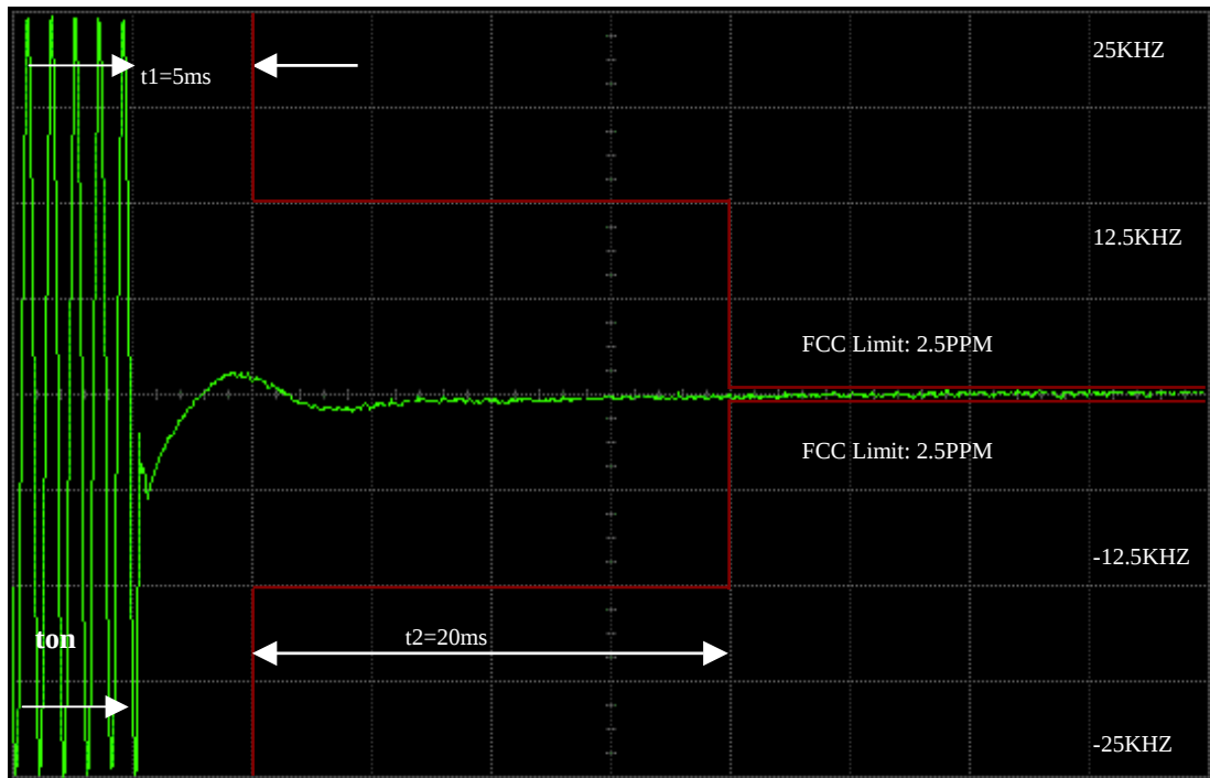
2 Watts, 173.975MHZ 25KHZ KEY-UP ATTACK TIME
