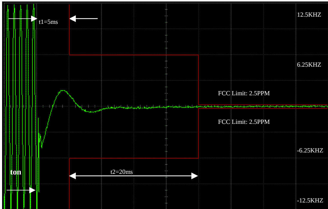
2 Watts, 162.025MHZ 12.5KHZ KEY-UP ATTACK TIME
