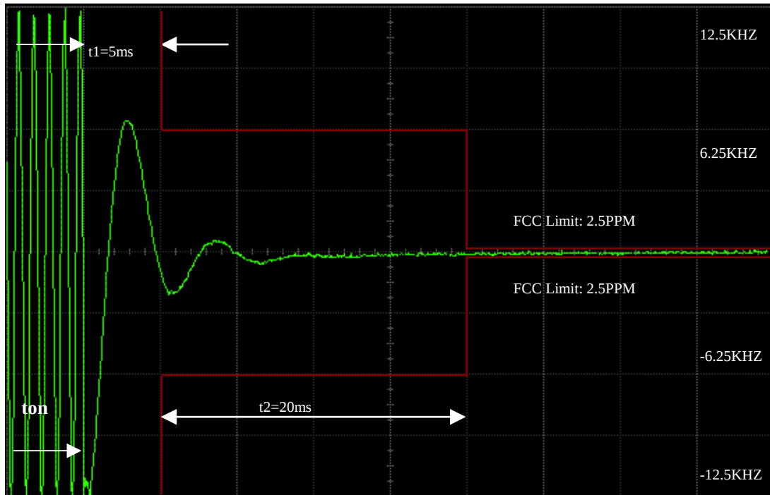
2 Watts, 148.025Mhz 12.5KHZ KEY-UP ATTACK TIME
