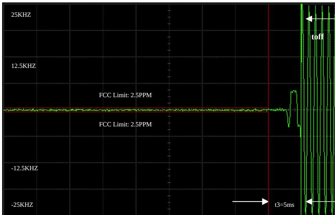
2 Watts, 173.975MHZ 25KHZ DE-KEY DECAY TIME
