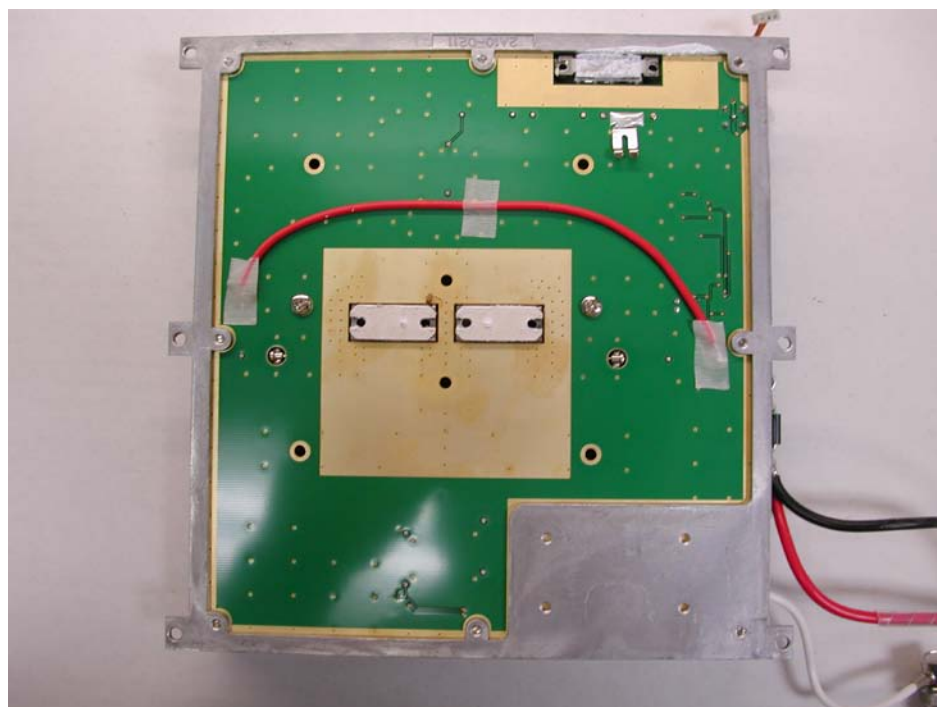
PA UNIT BOTTOM VIEW
