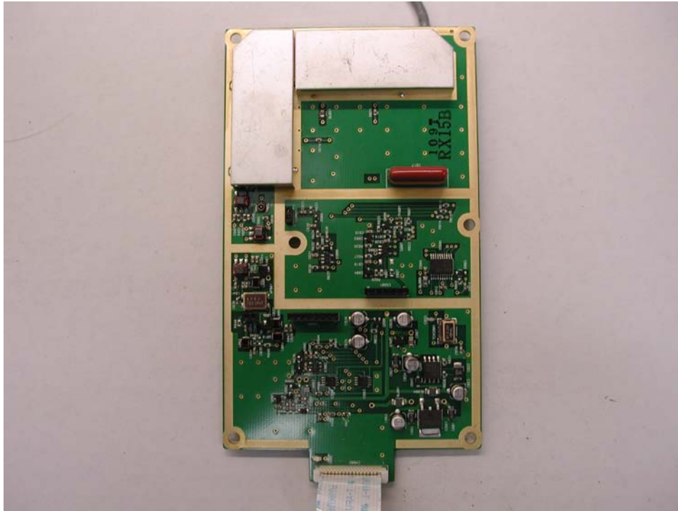
RX UNIT BOTTOM VIEW
