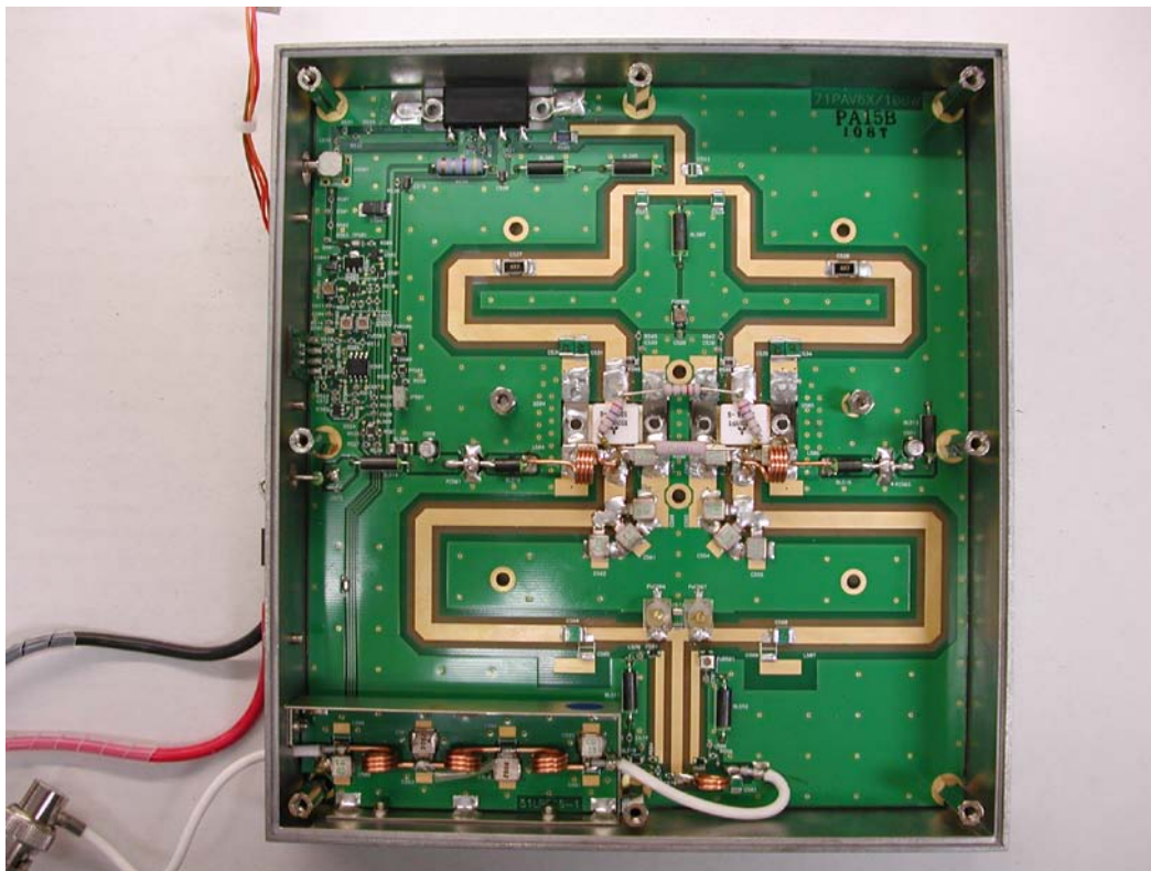
PA UNIT BOTTOM VIEW
