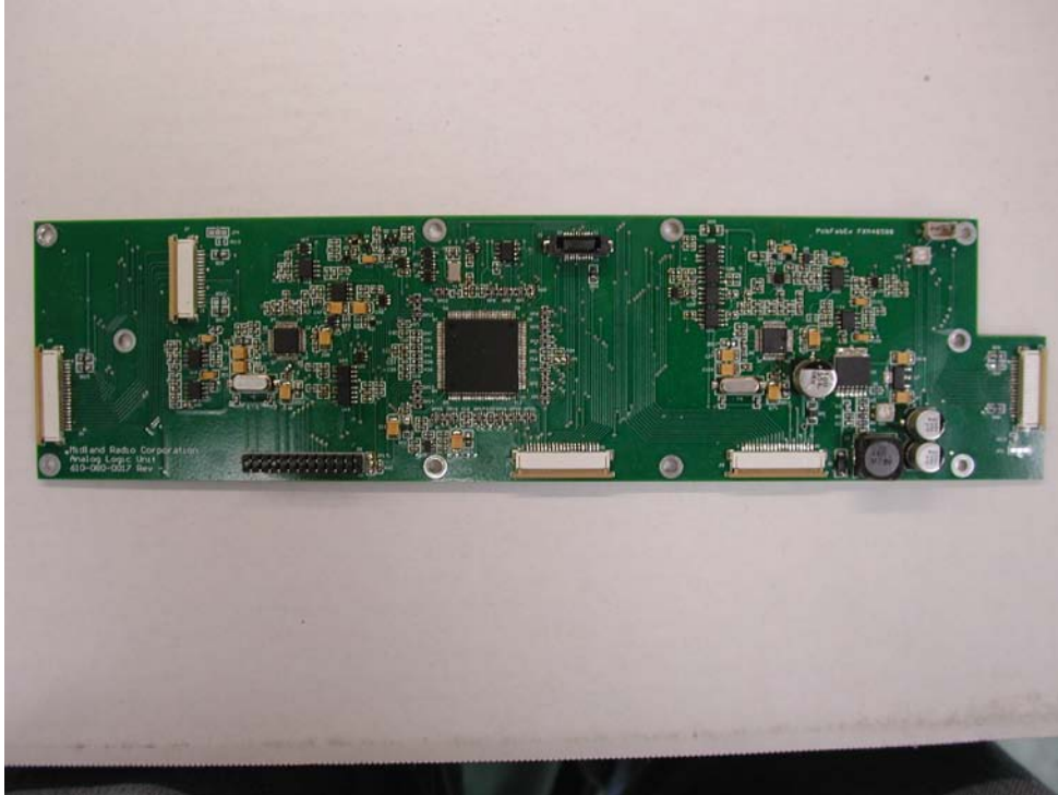
ANALOG LOG UNIT BOTTOM
