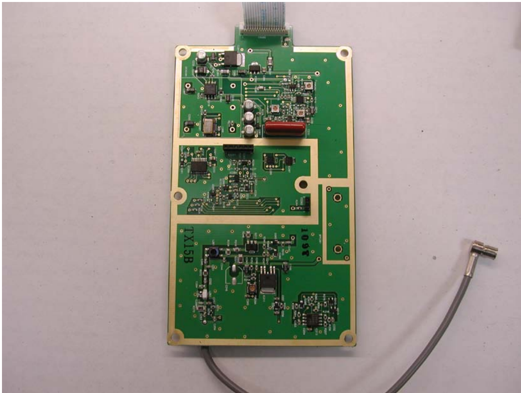
TX UNIT BOTTOM VIEW
