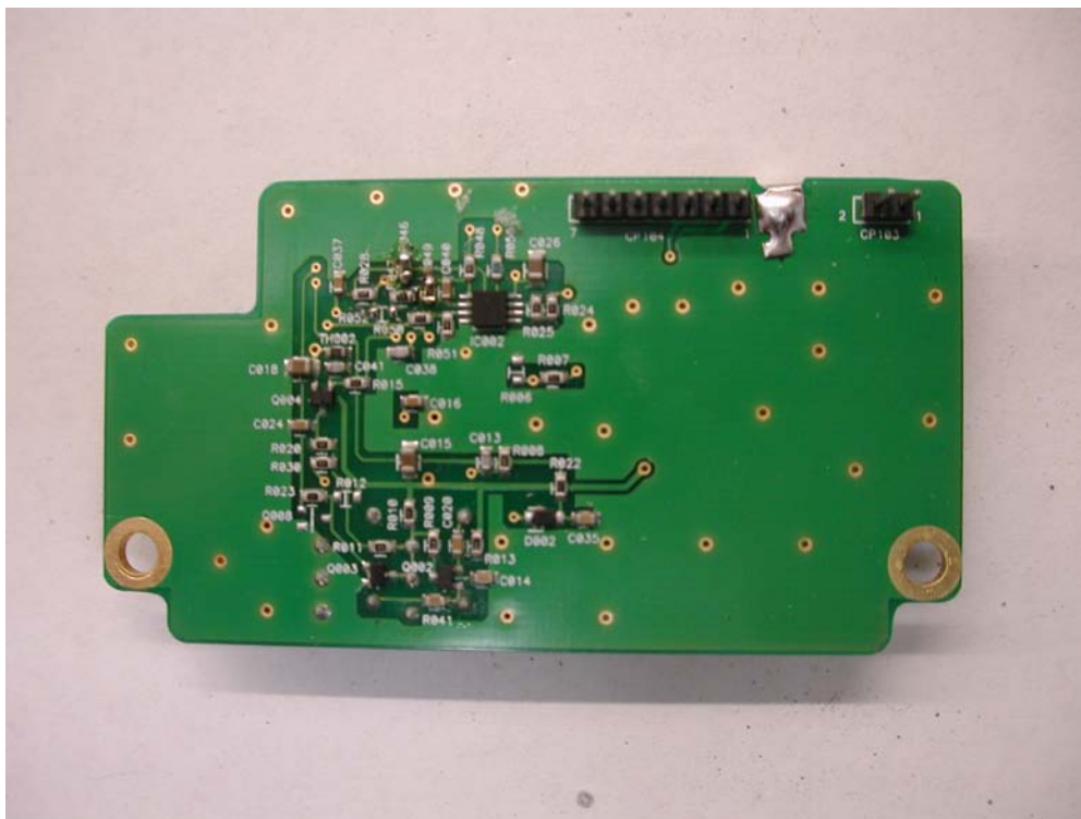
RX IF BOTTOM VIEW
