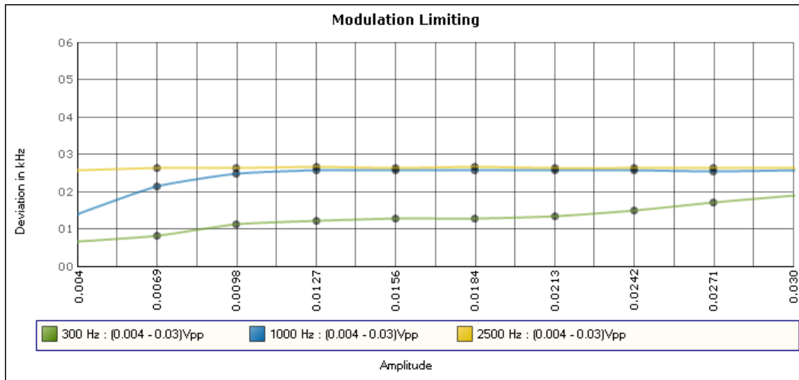
Modulation Limiting Plot
