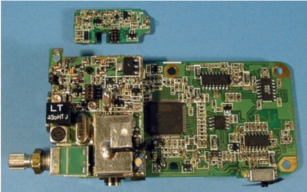
Main Board Top, and Small Daughter Board
