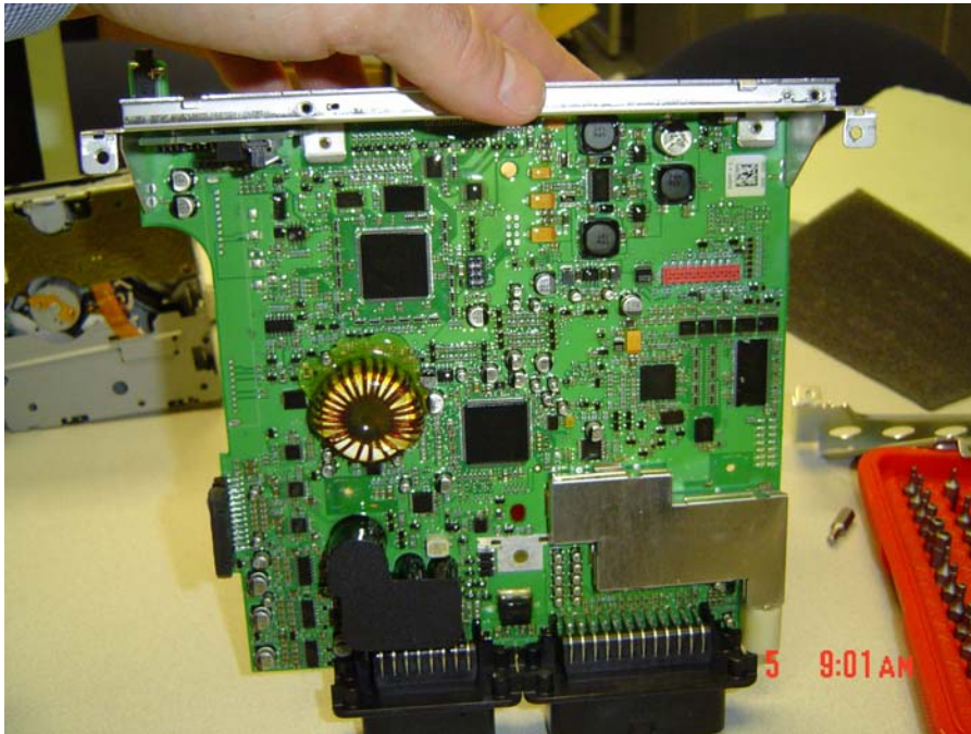
Head Unit – Main Board PCB Top View
