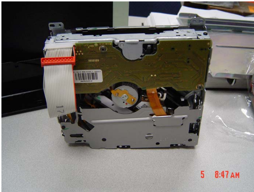
Head Unit – CD Mech Back View
