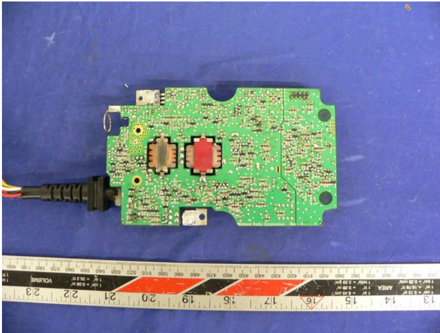
CB Radio – Board Solder View
