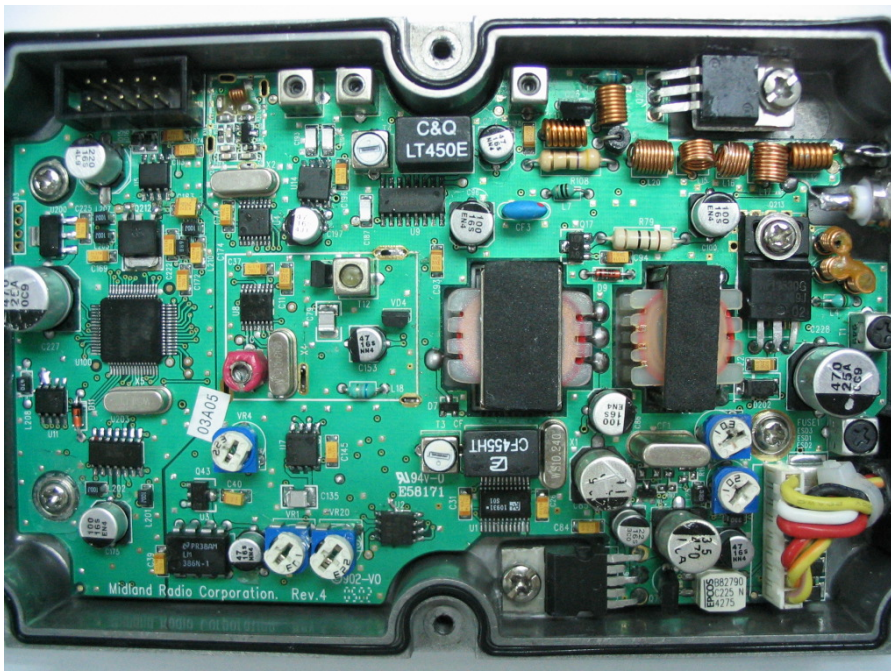
CB Radio – Board Transmitter View
