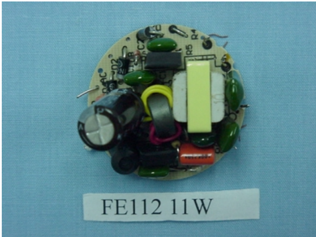
FIGURE 14 ENERGY SAVING LAMP (M/N: FE112 11W) MAIN BOARD (COMPONENT SIDE)
