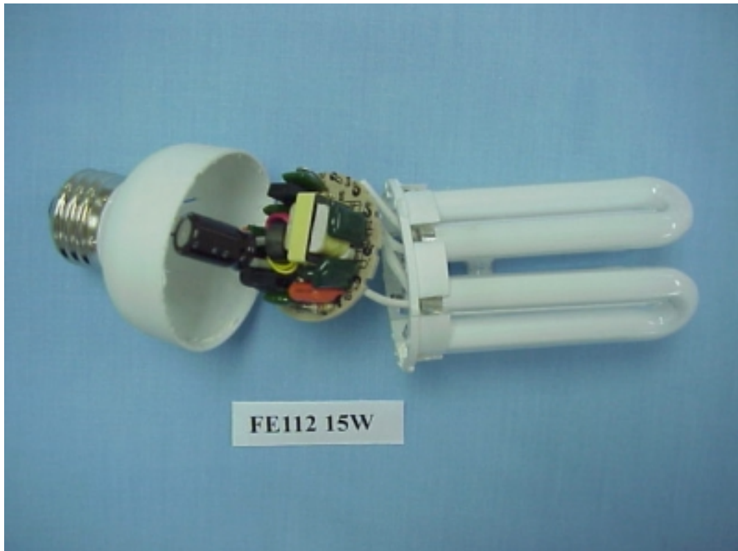
FIGURE 19 ENERGY SAVING LAMP (M/N: FE112 15W) COVER REMOVED
