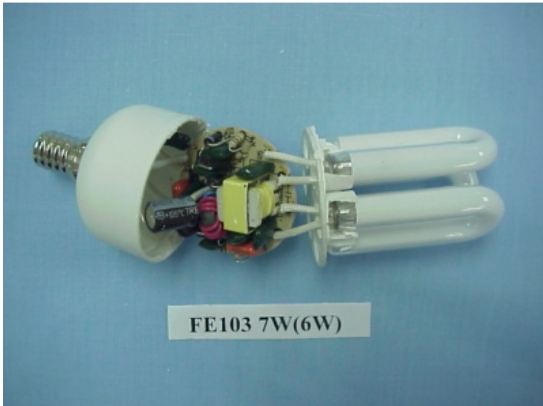
FIGURE 4 ENERGY SAVING LAMP (M/N: FE103 7W(6W)) COVER REMOVED
