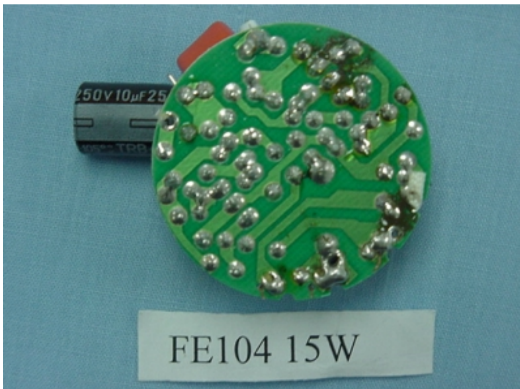
FIGURE 12 ENERGY SAVING LAMP (M/N: FE104 15W) MAIN BOARD (SOLDERED SIDE)
