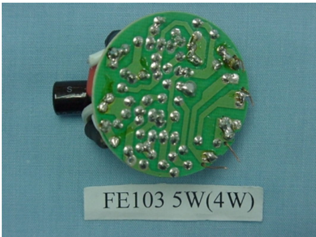
FIGURE 3 ENERGY SAVING LAMP (M/N: FE103 5W(4W)) MAIN BOARD (SOLDERED SIDE)
