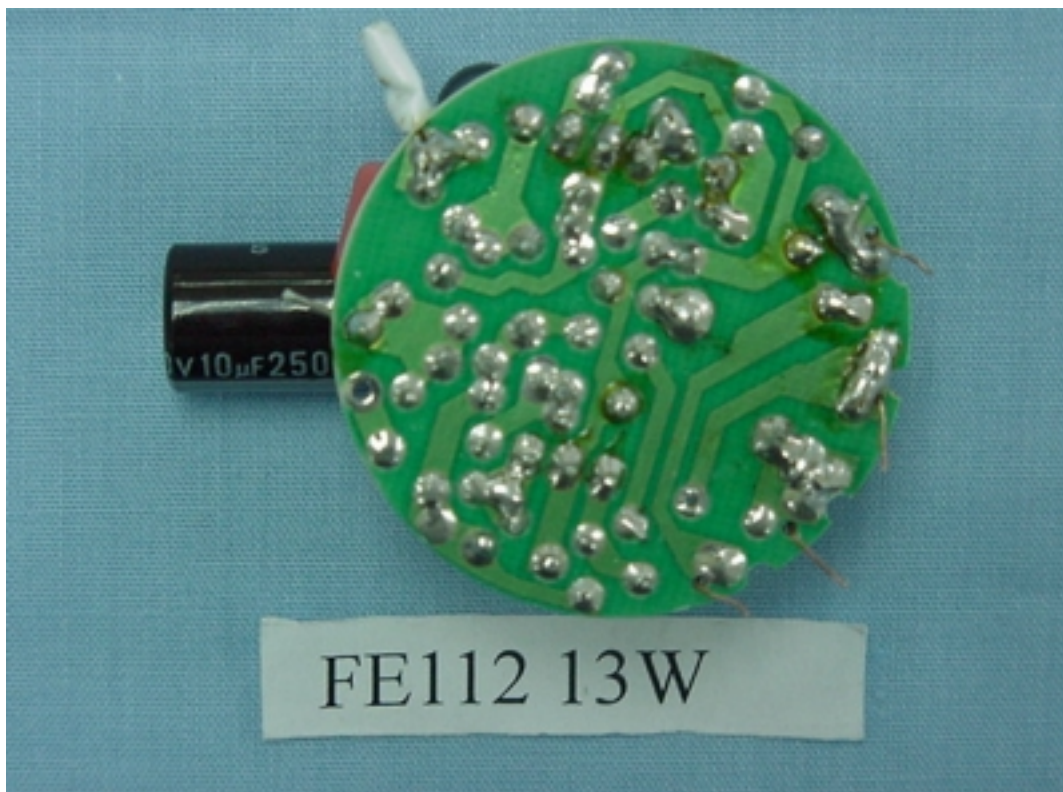
FIGURE 18 ENERGY SAVING LAMP (M/N: FE112 13W) MAIN BOARD (SOLDERED SIDE)
