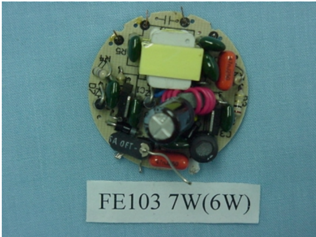
FIGURE 5 ENERGY SAVING LAMP (M/N: FE103 7W(6W)) MAIN BOARD (COMPONENT SIDE)
