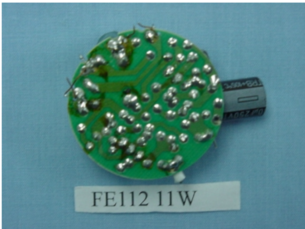
FIGURE 15 ENERGY SAVING LAMP (M/N: FE112 11W) MAIN BOARD (SOLDERED SIDE)
