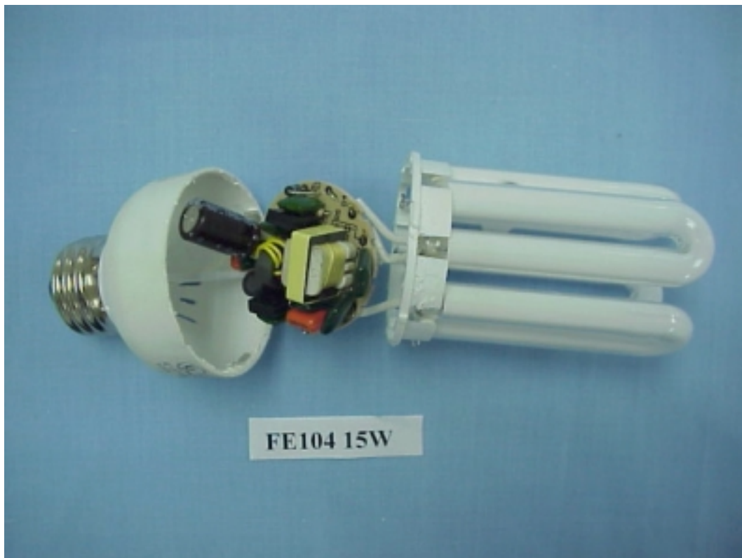
FIGURE 10 ENERGY SAVING LAMP (M/N: FE104 15W) COVER REMOVED
