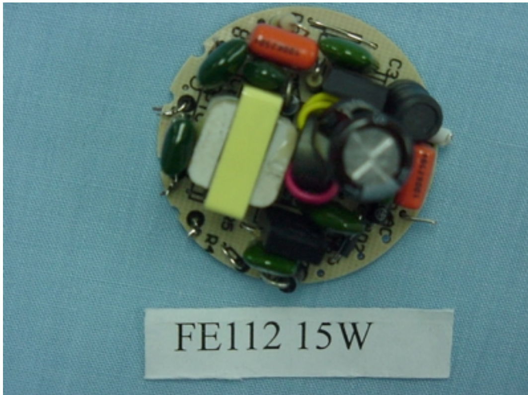
Figure 20 ENERGY SAVING LAMP (M/N: FE112 15W) MAIN BOARD (COMPONENT SIDE)
