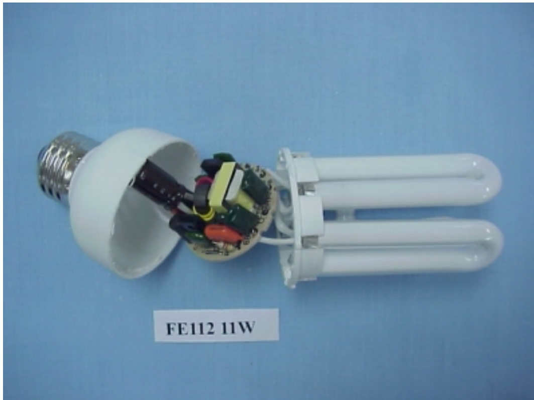
FIGURE 13 ENERGY SAVING LAMP (M/N: FE112 11W) COVER REMOVED
