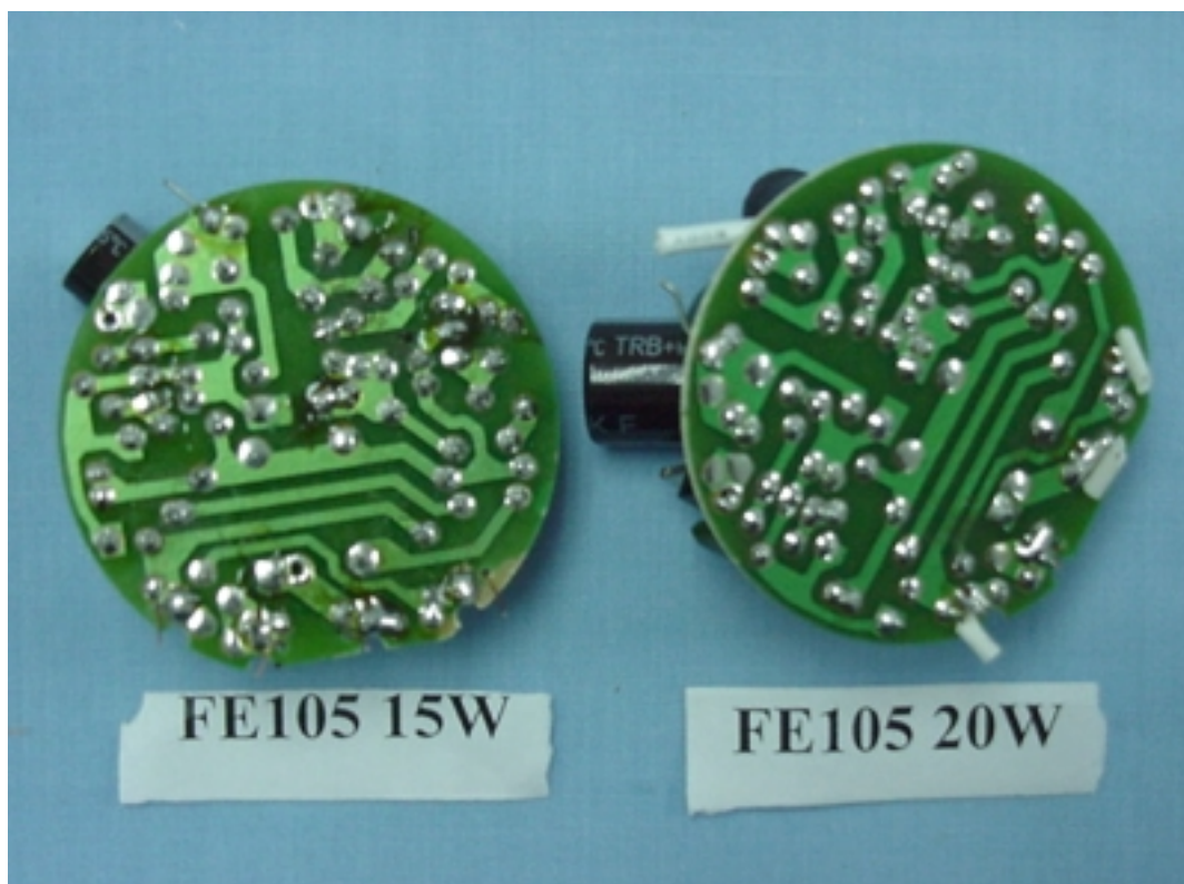
FIGURE 21 ENERGY SAVING LAMP (M/N: FE105 15W & FE105 20W) MAIN BOARD (SOLDERED SIDE)
