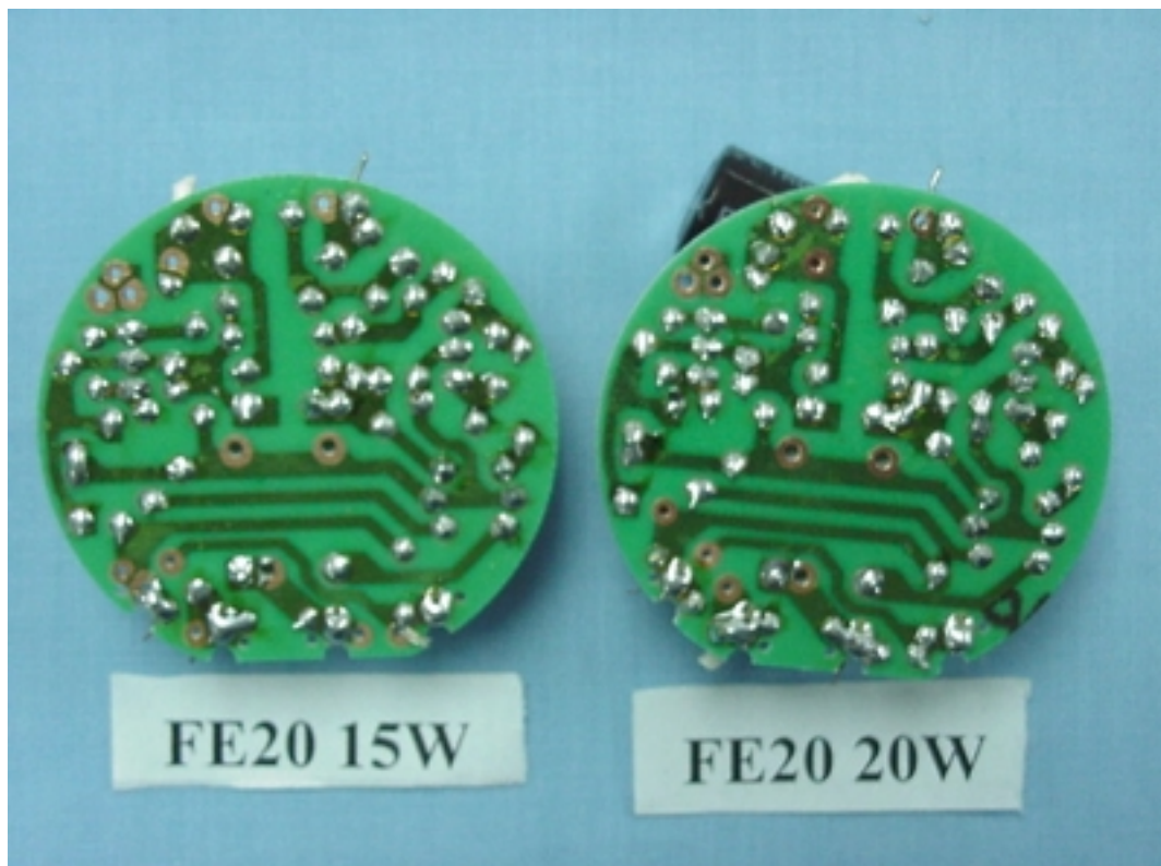
FIGURE 3 ENERGY SAVING LAMP (M/N: FE20 15W & FE20 20W) MAIN BOARD (SOLDERED SIDE)
