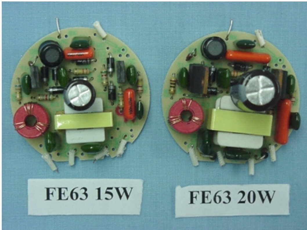
Figure 8 ENERGY SAVING LAMP (M/N: FE63 15W & FE63 20W) MAIN BOARD (COMPONENT SIDE)
