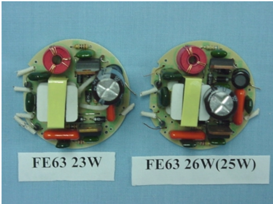
Figure 11 ENERGY SAVING LAMP (M/N: FE63 23W & FE63 26W(25W)) MAIN BOARD (COMPONENT SIDE)
