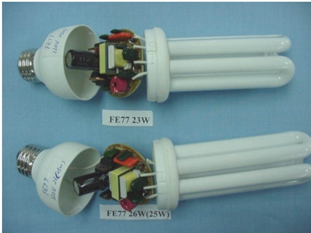
FIGURE 16 ENERGY SAVING LAMP (M/N: FE77 23W & FE77 26W(25W)) COVER REMOVED
