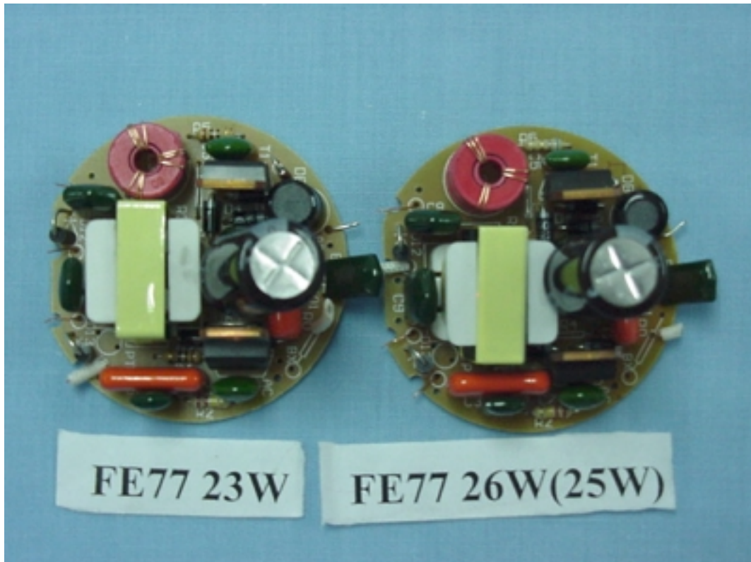
FIGURE 17 ENERGY SAVING LAMP (M/N: FE77 23W & FE77 26W(25W)) MAIN BOARD (COMPONENT SIDE)
