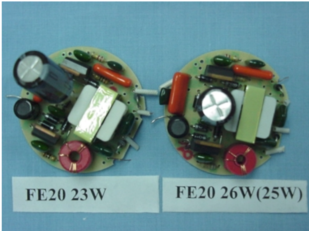
Figure 5 ENERGY SAVING LAMP (M/N: FE20 23W & FE20 26W(25W)) MAIN BOARD (COMPONENT SIDE)
