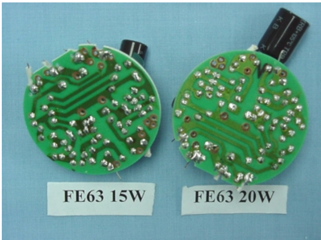
FIGURE 9 ENERGY SAVING LAMP (M/N: FE63 15W & FE63 20W) MAIN BOARD (SOLDERED SIDE)
