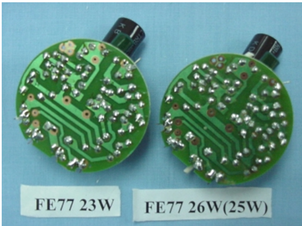
FIGURE 18 ENERGY SAVING LAMP (M/N: FE77 23W & FE77 26W(25W)) MAIN BOARD (SOLDERED SIDE)
