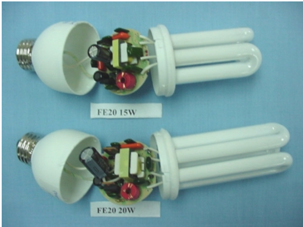
FIGURE 1 ENERGY SAVING LAMP (M/N: FE20 15W & FE20 20W) COVER REMOVED
