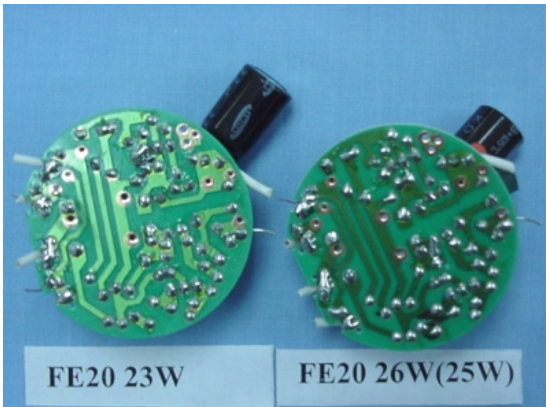
FIGURE 6 ENERGY SAVING LAMP (M/N: FE20 23W & FE20 26W(25W)) MAIN BOARD (SOLDERED SIDE)
