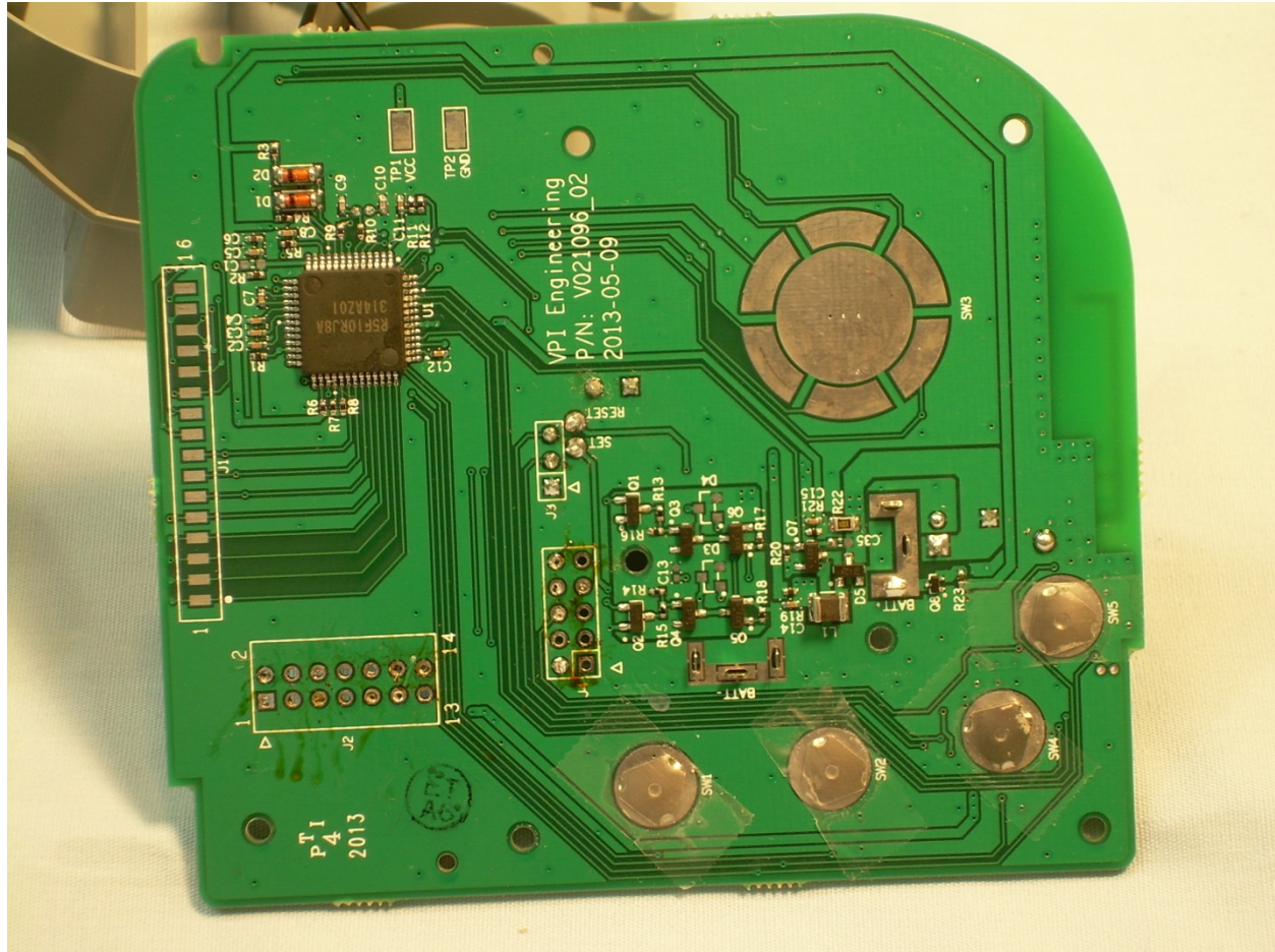
View of the Front Side of the PCB
