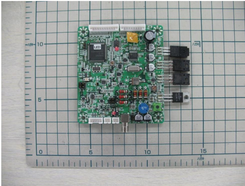
TR3-L201W4 without Shieling
