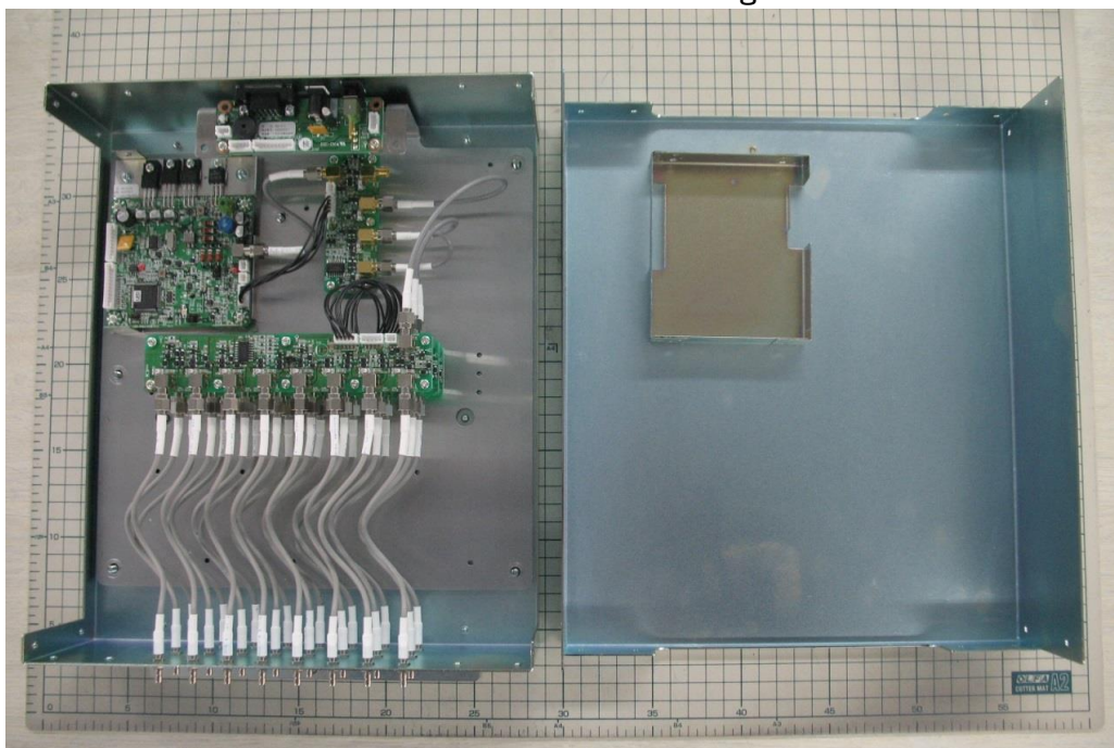
TR3-L4D01-24 without Shielding
