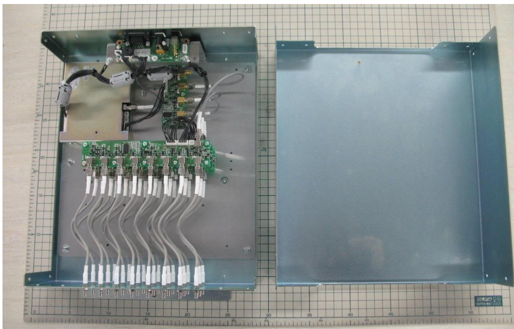
TR3-L4D01-24 in Case
