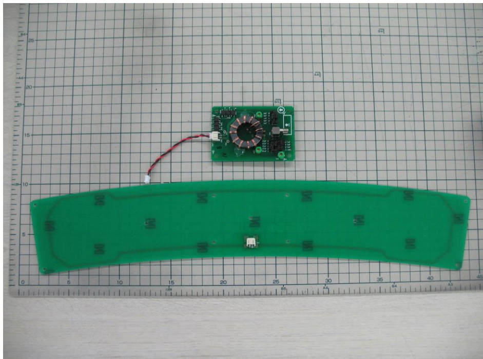
Bottom View
