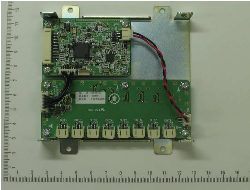
TR3-C202 and TR3-PS202 in Case
