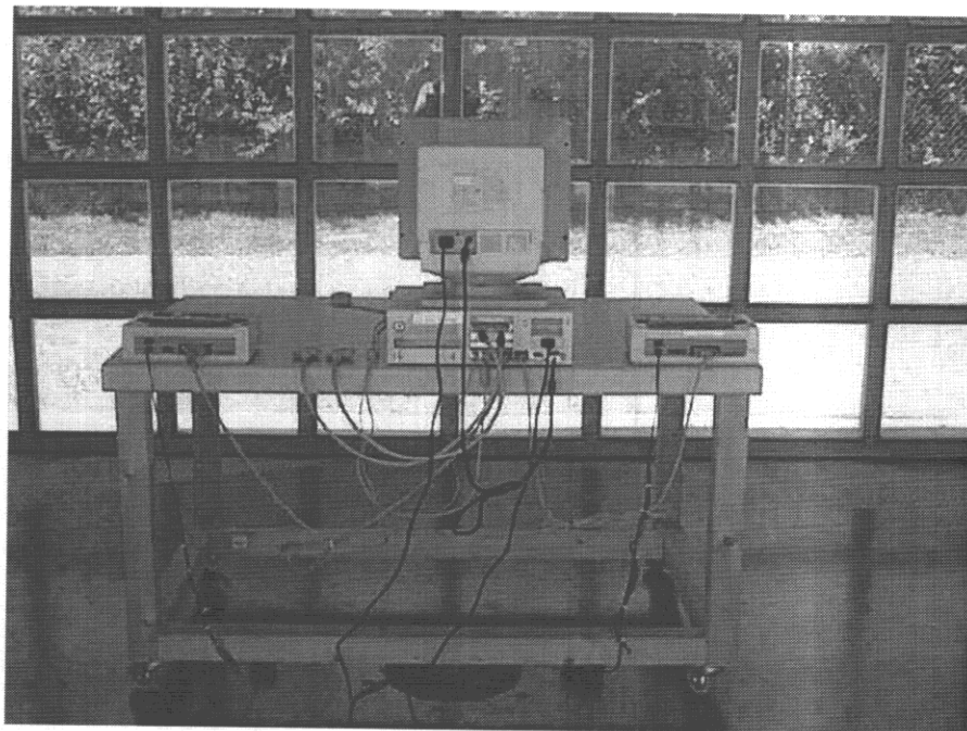
Back view of radiated measurements
