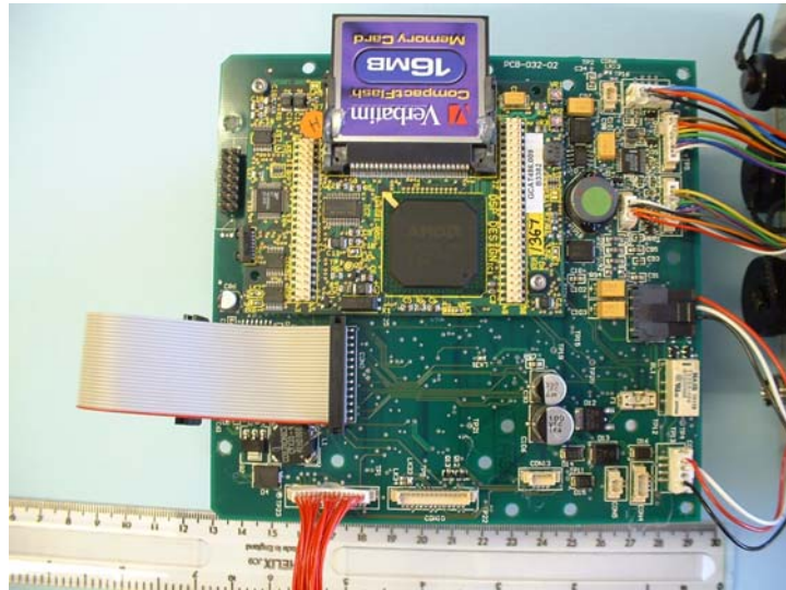
PCB TRACK SIDE
