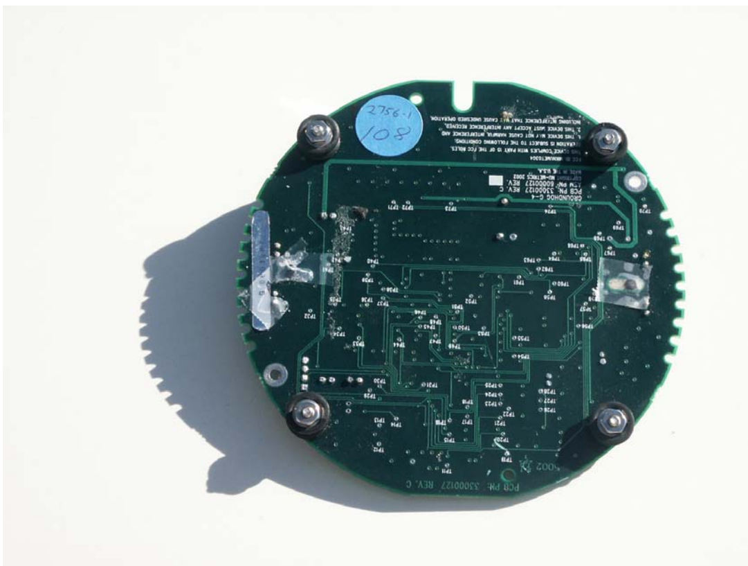
PCB Back
