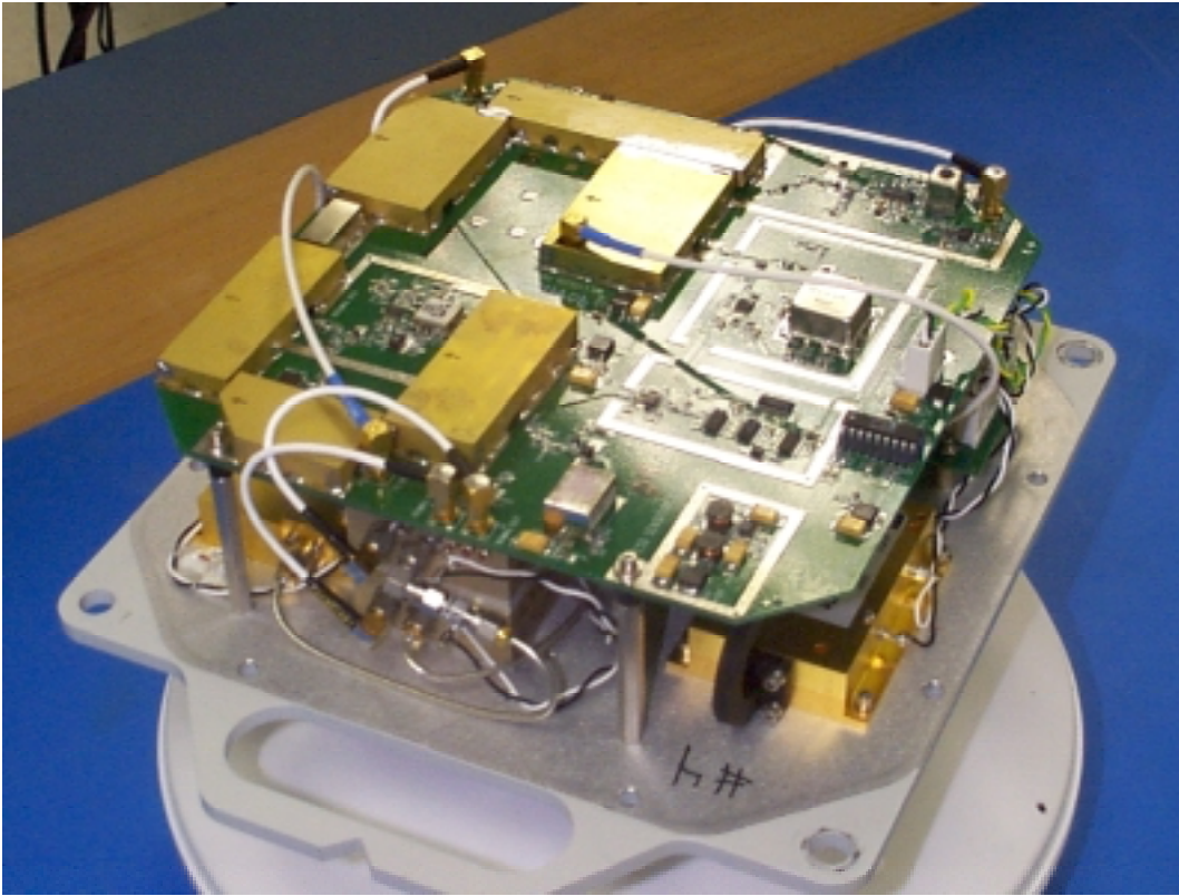
Figure 11.0-2 CPE Internal View
