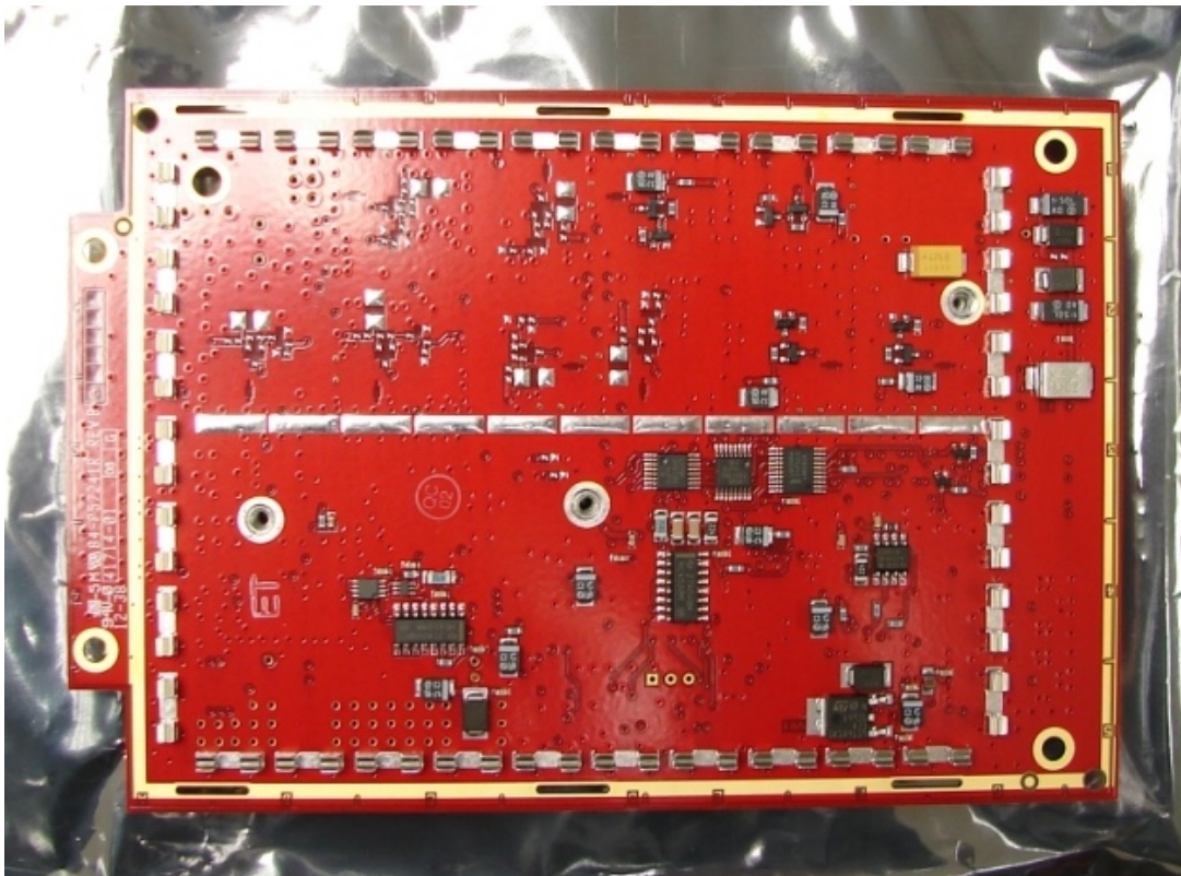
Figure 9.0-17 SVHF CCA Back without Shield
