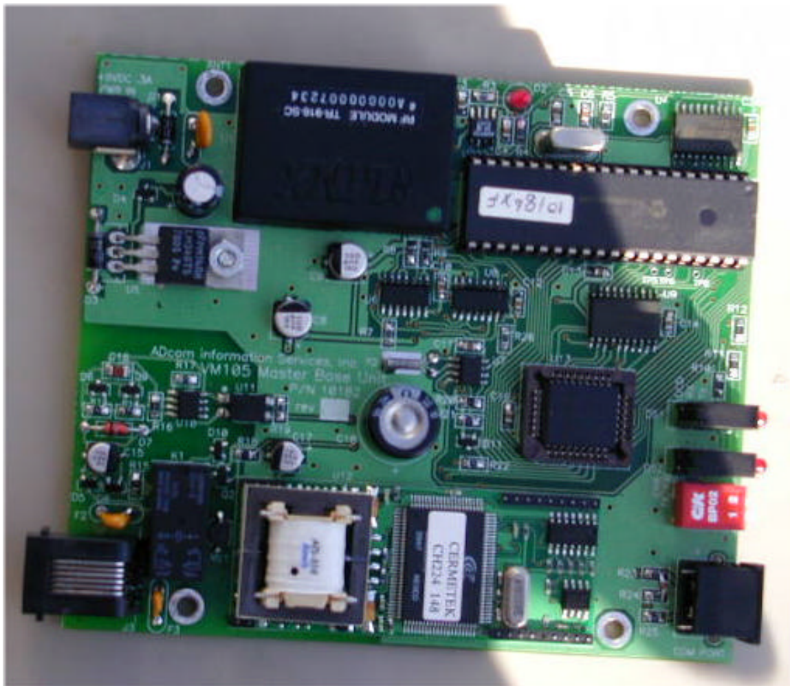
BOARD TOP
