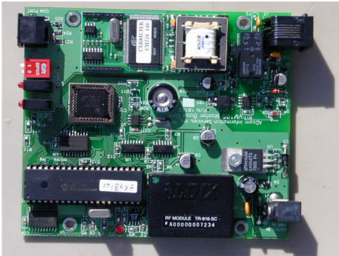
BOARD TOP
