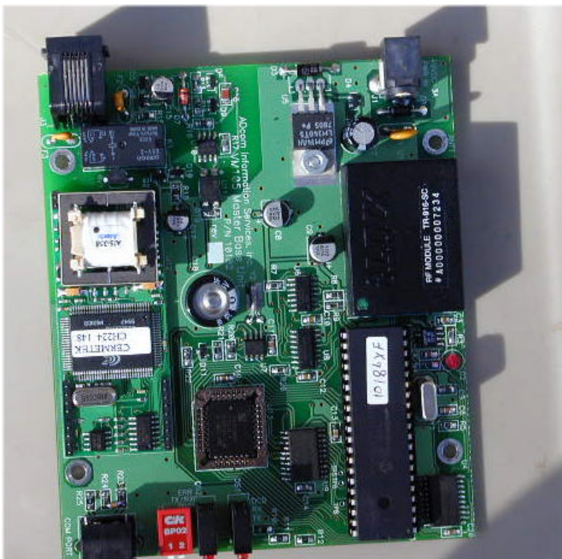
BOARD TOP
