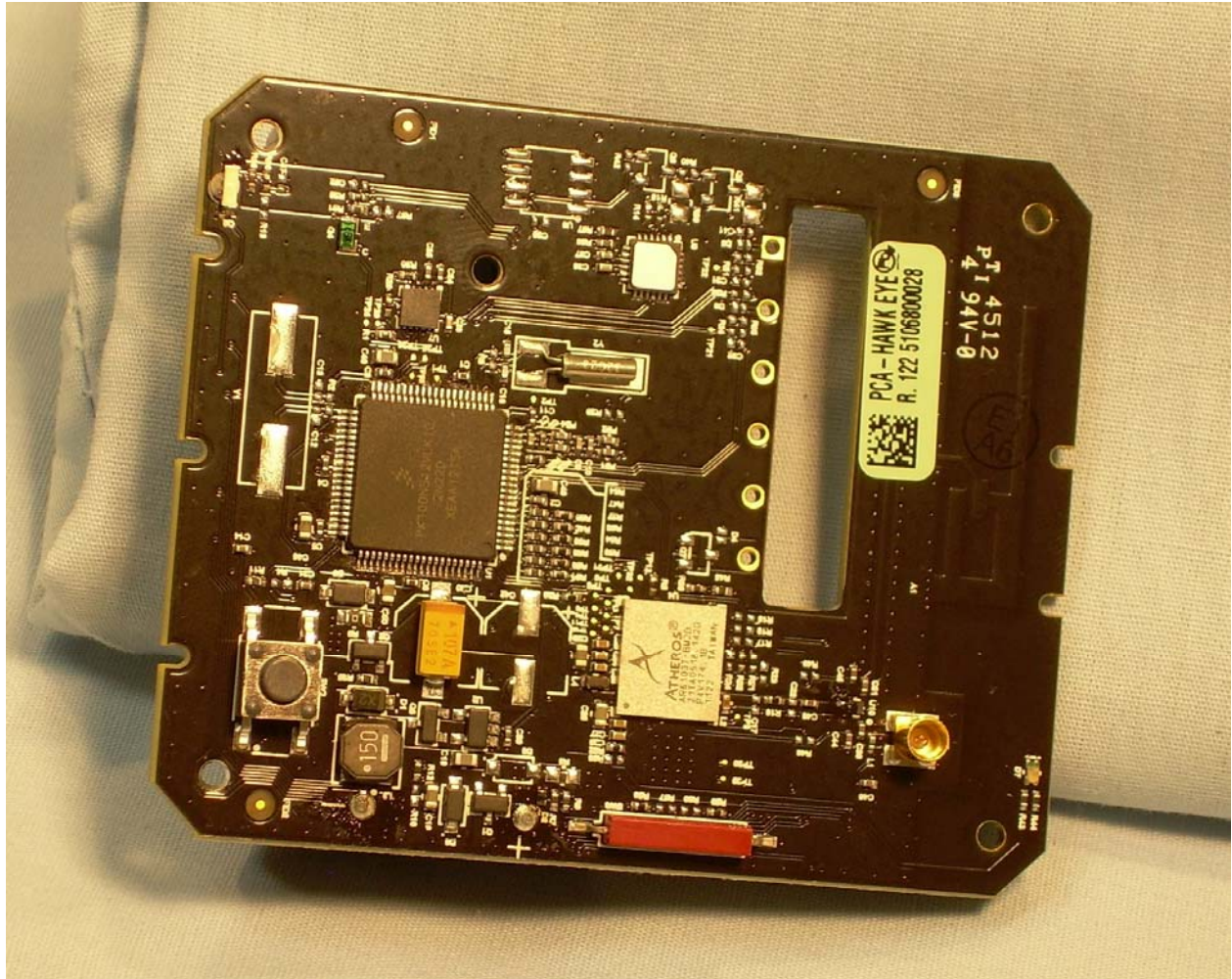
View of the Front Side of the EUT PCB
