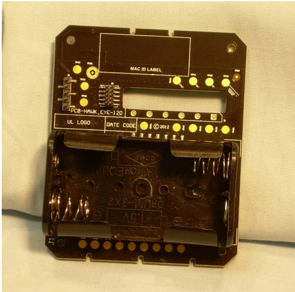
View of the Front Side of the EUT PCB
