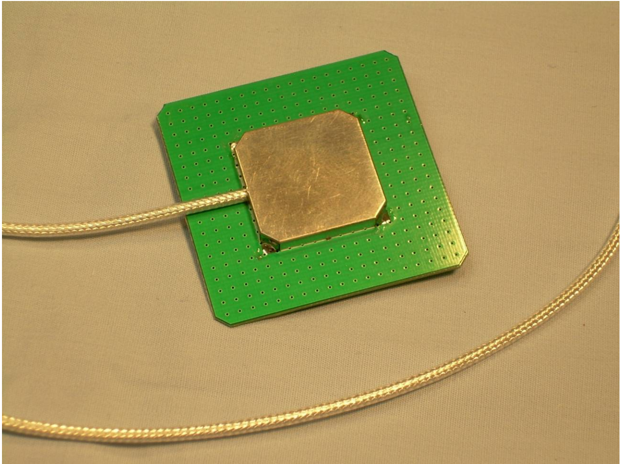
View of the Back Side of the External Antenna
