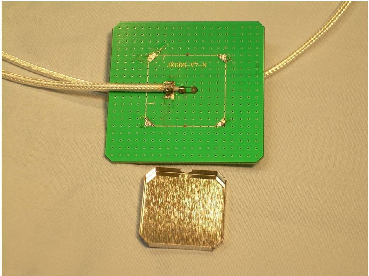
View of the Back Side of the External Antenna with Cover Removed
