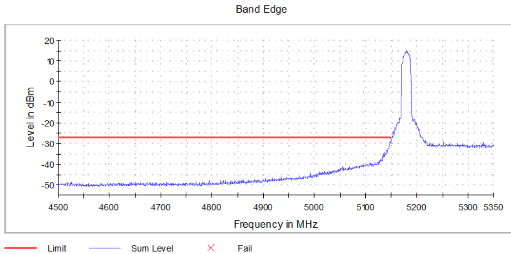
Graph 11: Lower Band Edge Channel 36 Transmitting
