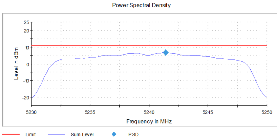
Graph 9: Conducted Power Transmitting at 5240 MHz
