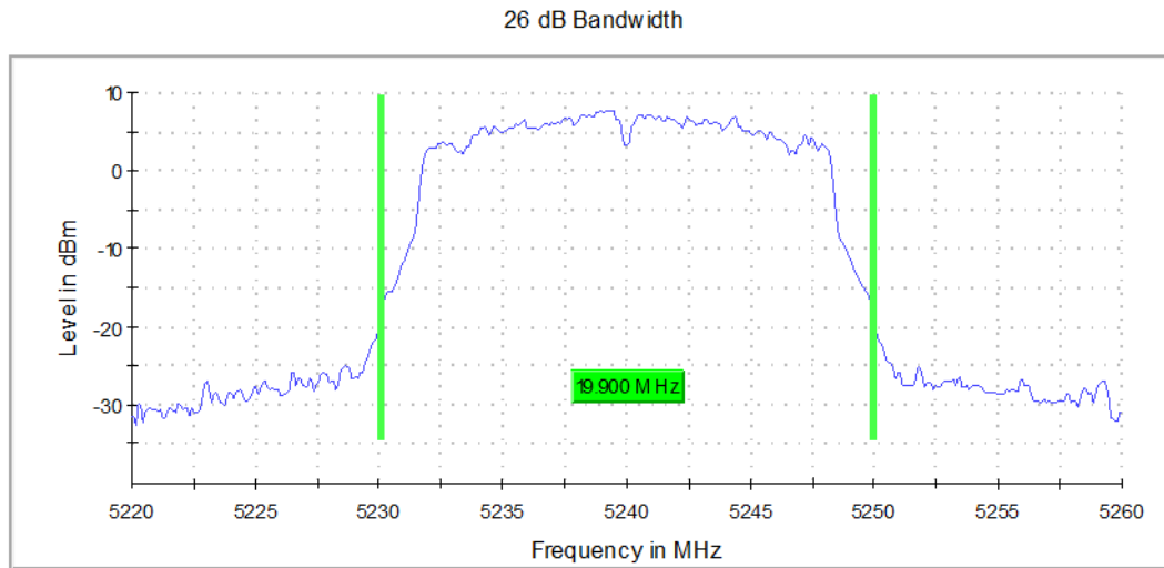
Graph 3: 26 dB Emissions Bandwidth Transmitting at 5240 MHz
