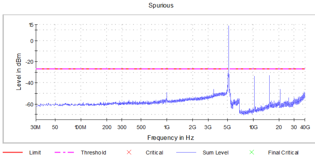
Graph 13: Spurious Emissions Channel 40 Transmitting
