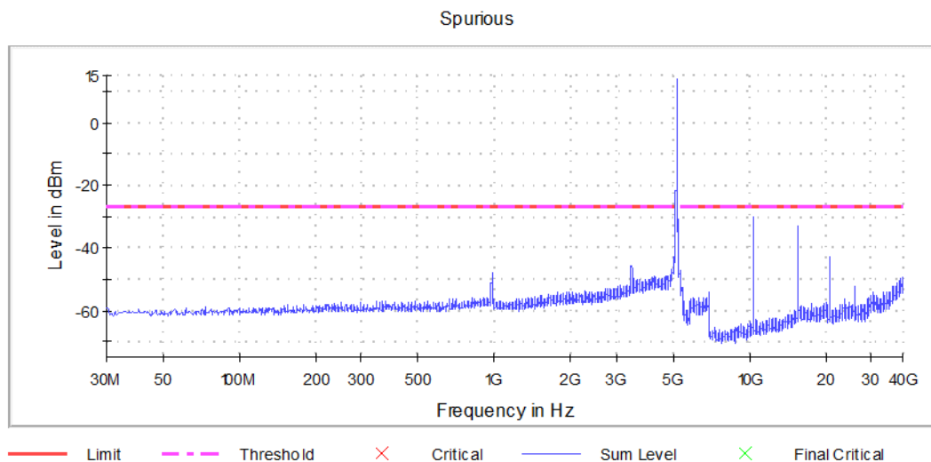
Graph 12: Spurious Emissions Channel 36 Transmitting
