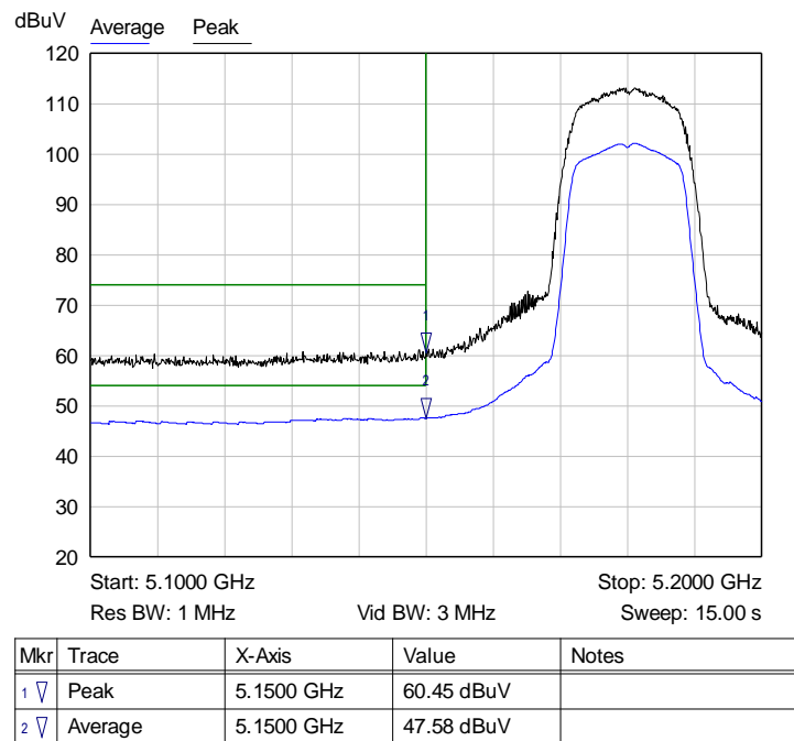
Graph 10: Channel 36 Band Edge at the Restricted Band Plot
