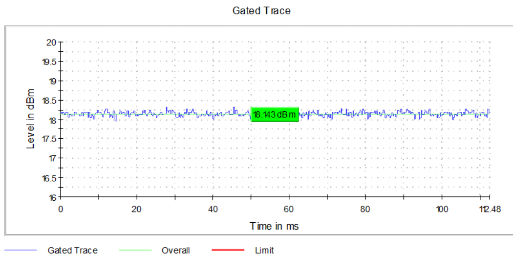
Graph 6: Conducted Power Transmitting at 5240 MHz
