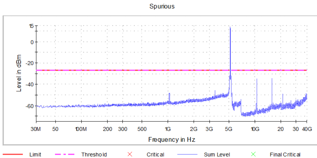
Graph 14: Spurious Emissions Channel 48 Transmitting
