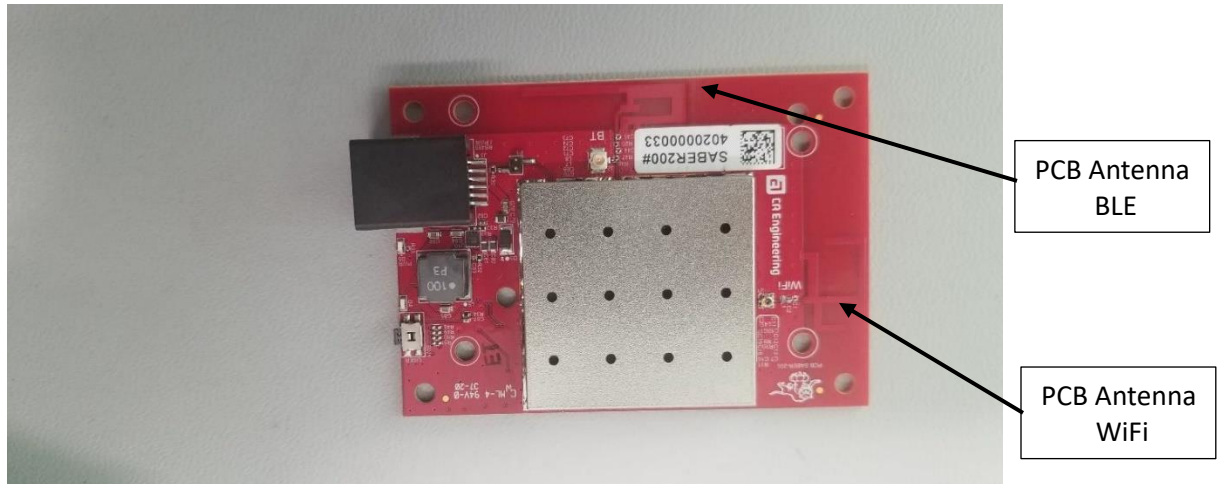
Photograph 1 – Top View of the PCB with Shield
