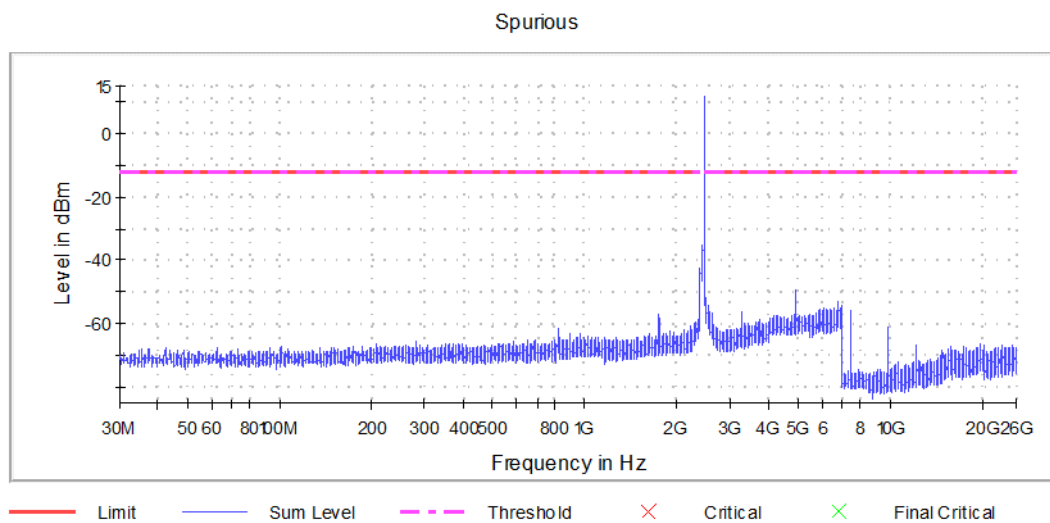
Graph 9: Transmitting on the Highest Channel
