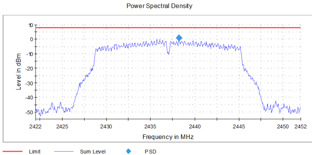
Graph 47: Middle Channel 3 kHz PSD Plot
