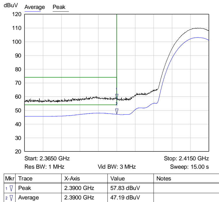
Graph 12: Radiated Lower Band Edge Plot
