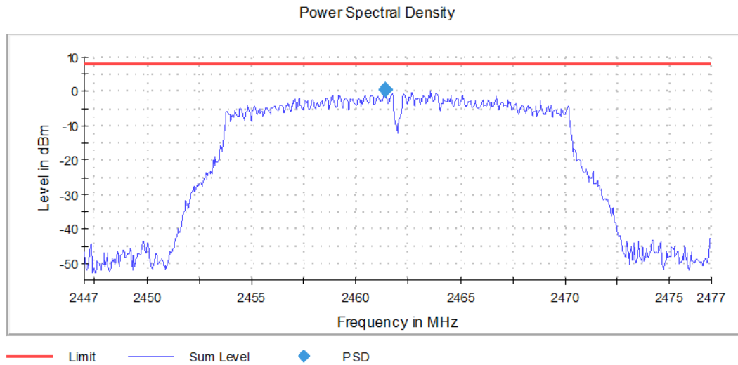
Graph 32: Highest Channel Output PSD Plot
