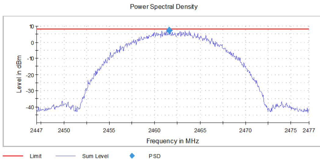
Graph 16: Highest Channel Output PSD Plot
