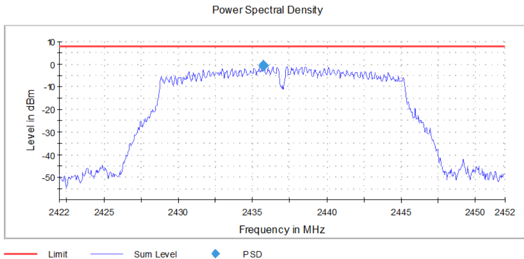
Graph 31: Middle Channel PSD Plot
