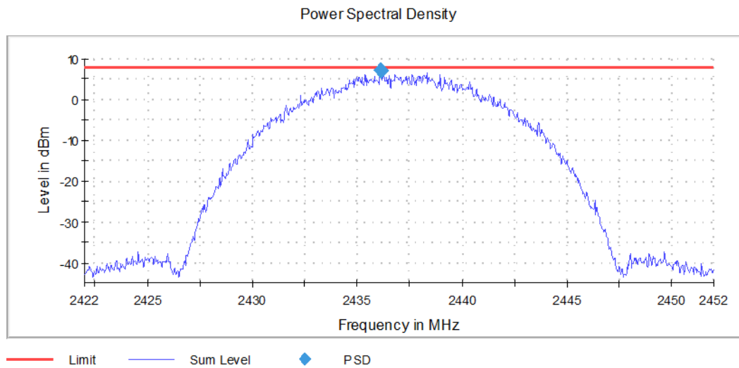
Graph 15: Middle Channel PSD Plot
