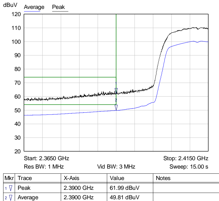
Graph 28: Radiated Lower Band Edge Plot
