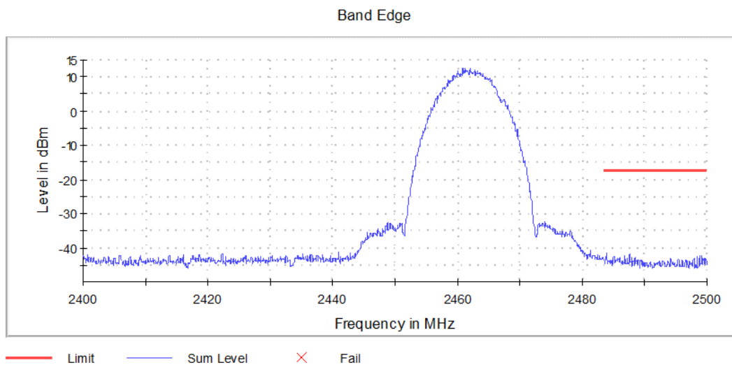
Graph 11: Upper Band Edge Plot
