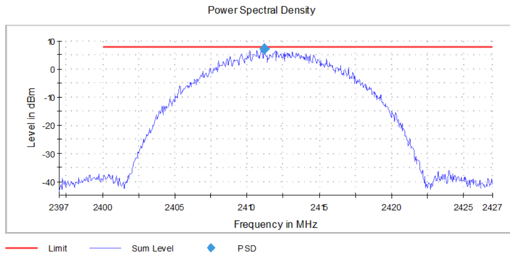
Graph 14: Lowest Channel PSD Plot
