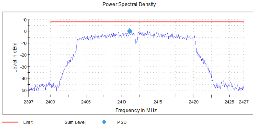
Graph 30: Lowest Channel PSD Plot
