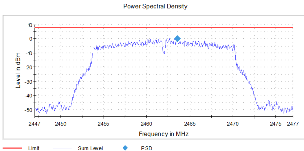
Graph 48: Highest Channel Output 3 kHz PSD Plot
