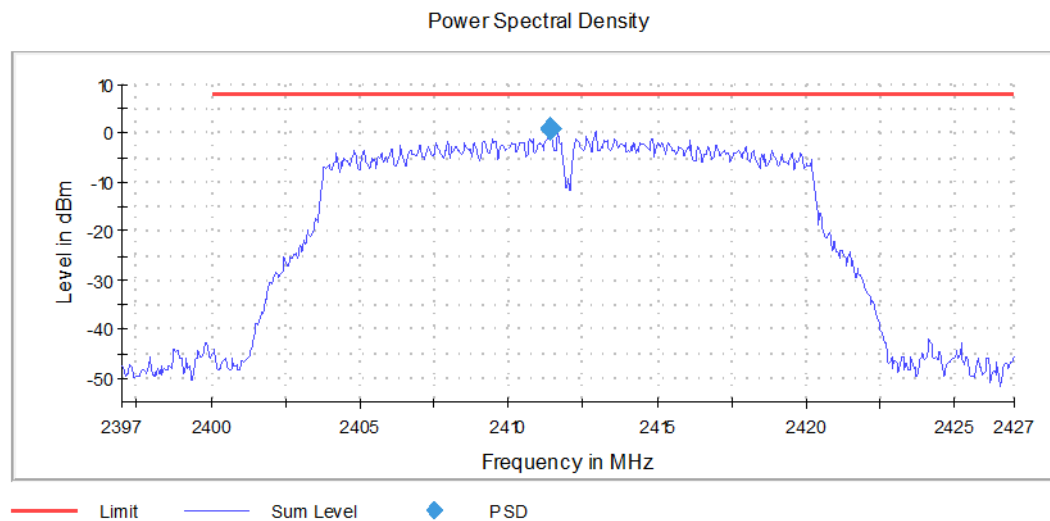
Graph 46: Lowest Channel 3 kHz PSD Plot
