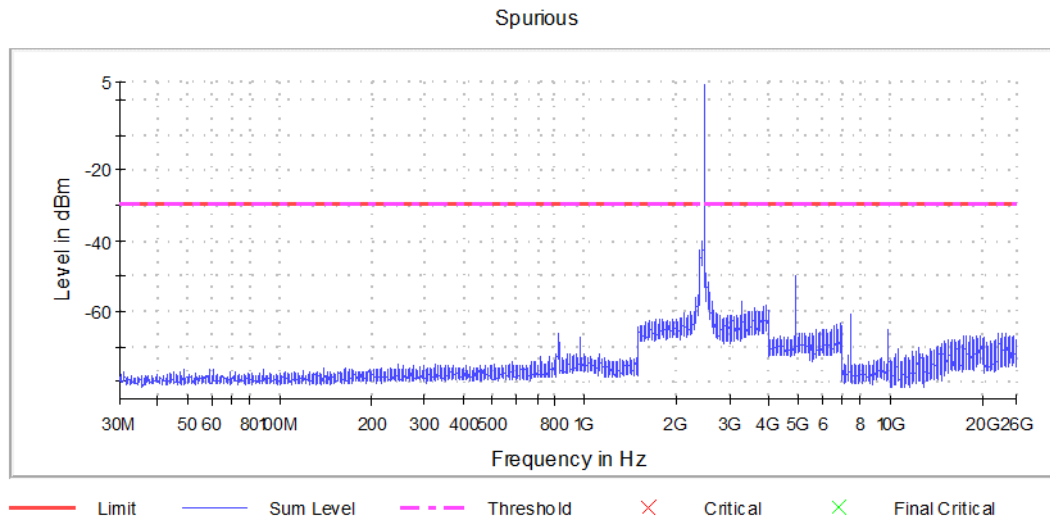
Graph 25: Transmitting on the Highest Channel
