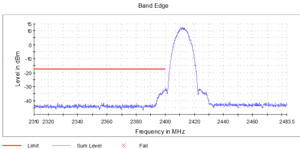
Graph 10: Lower Band Edge Plot
