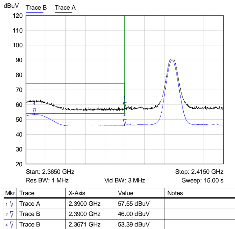
Graph 9: Radiated Lower Band Edge Plot
