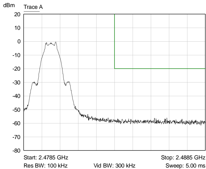
Graph 8: Upper Band Edge Plot
